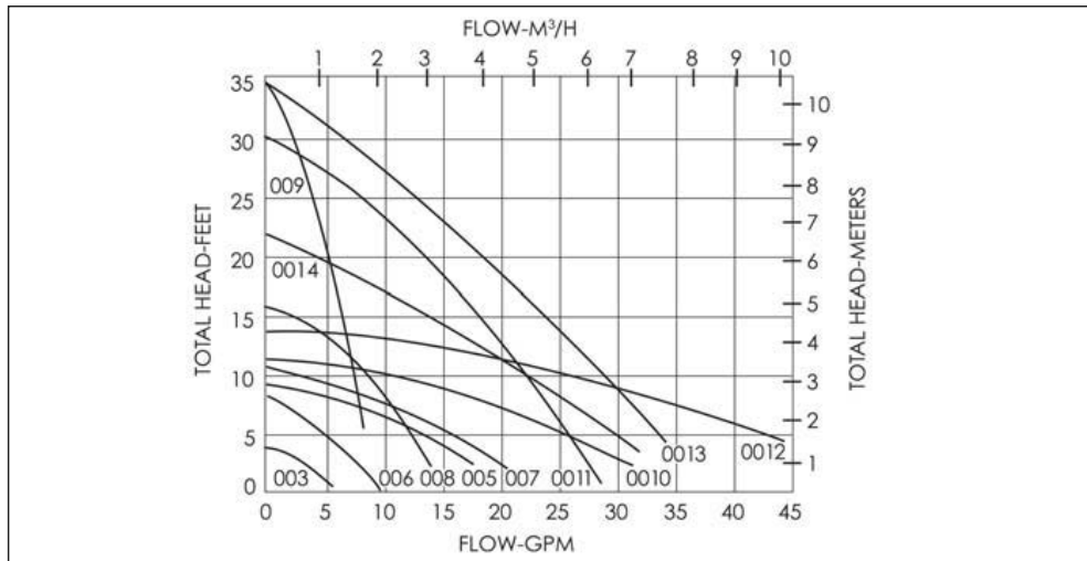
Figure 3: Taco 00 Series performance curves
