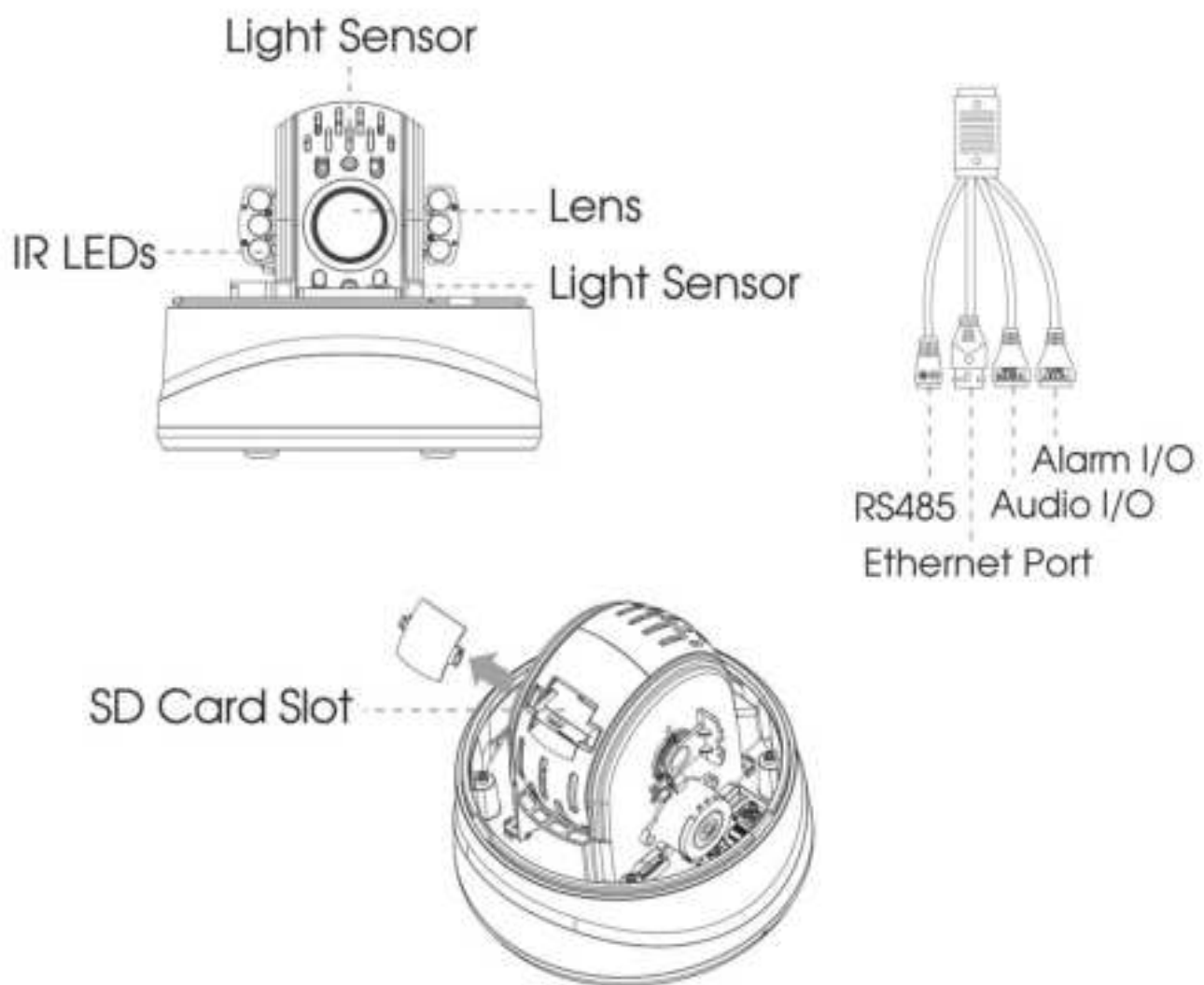
Figure 1-3-4 (AI) 12X/20X/23X Mini PTZ Dome Network Camera
