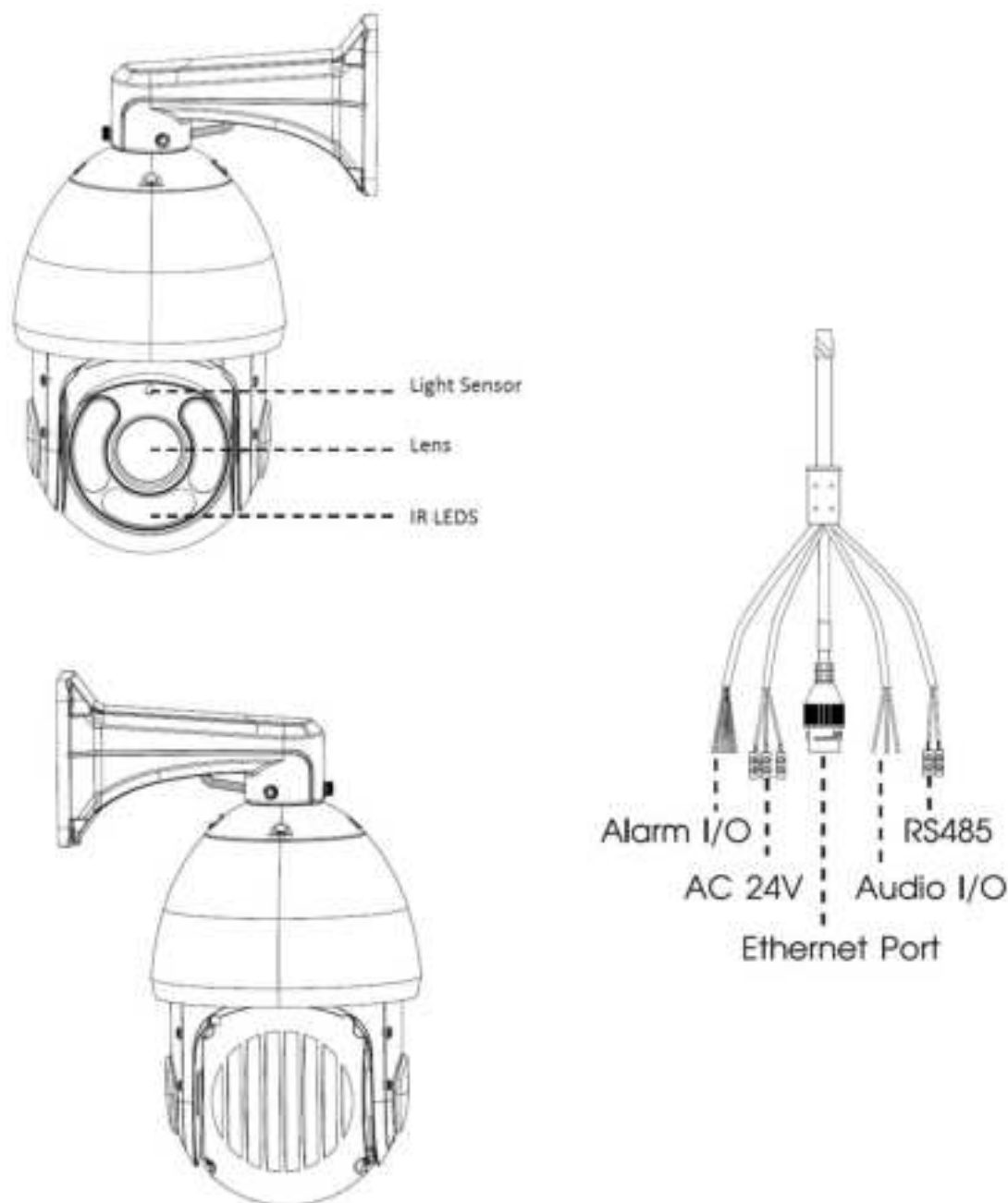
Figure 1-3-1 23X/30X/36X/42X Speed Dome Network Camera
