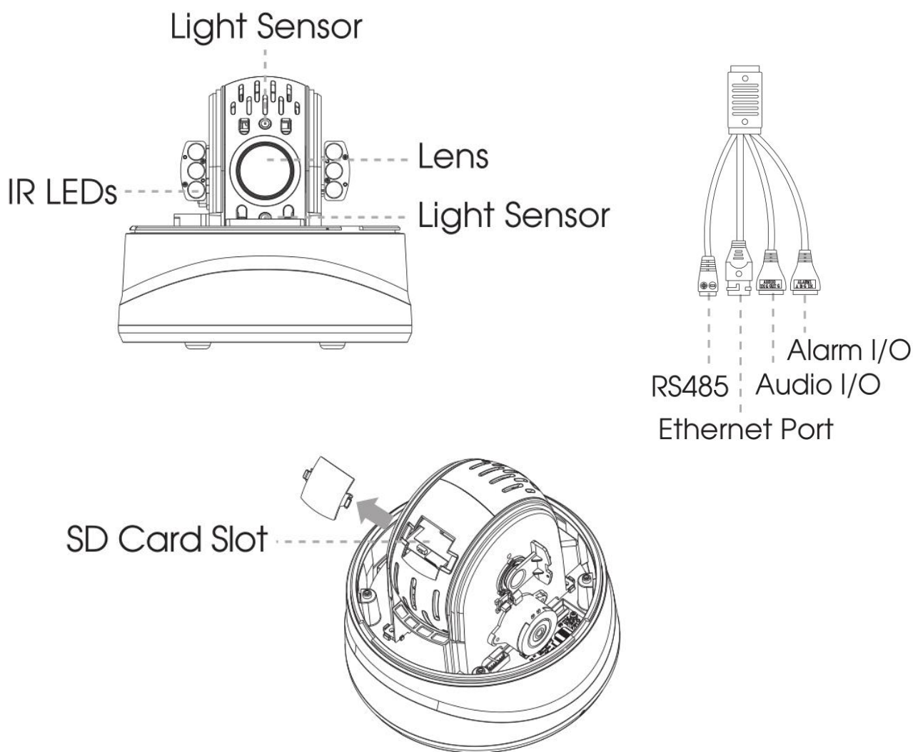
Figure 1-3-4 (AI) 12X/20X/23X Mini PTZ Dome Network Camera
