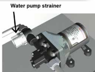
Water Pump Strainer
