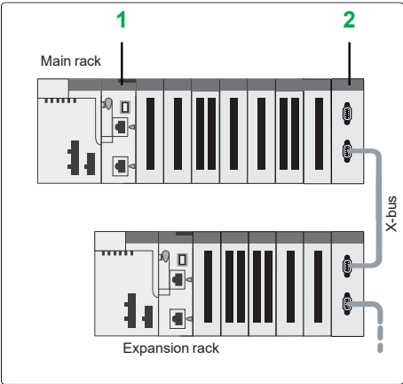
Local I/O architecture
