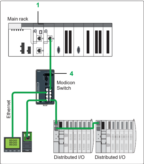
Distributed I/O architecture with BMXNOE0110
