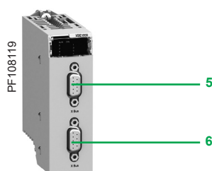
Rack expansion module BMXXBE1000
