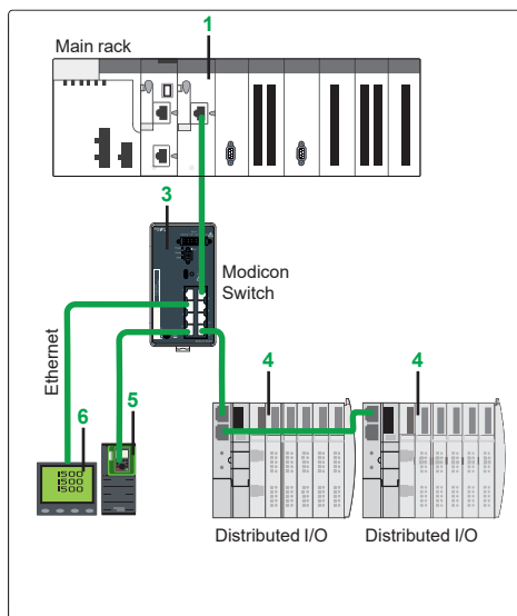
Distributed I/O architecture: devices distributed over Ethernet with BMXNOE0110 module and Modicon Switch
