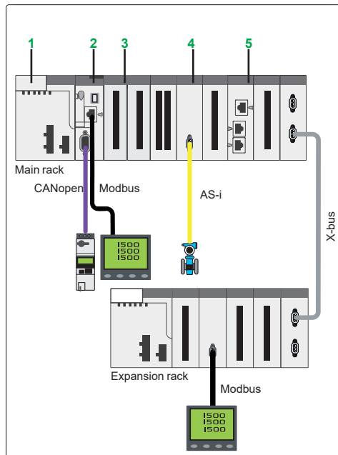
Integrated fieldbus architecture: devices distributed over fieldbuses
