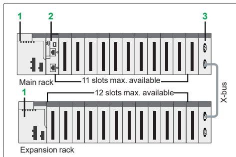
Local I/O architecture
