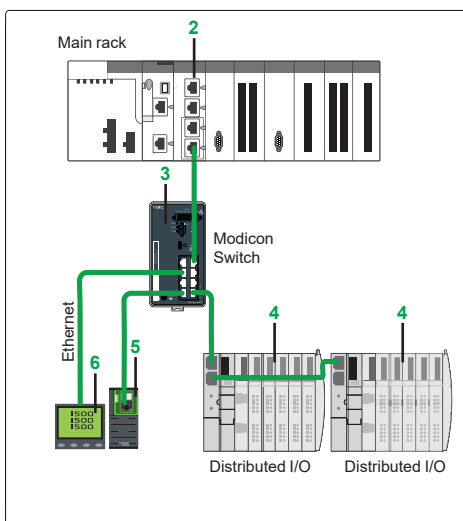
Distributed I/O architecture: devices distributed over Ethernet with BMXNOC0401 module and Modicon Switch
