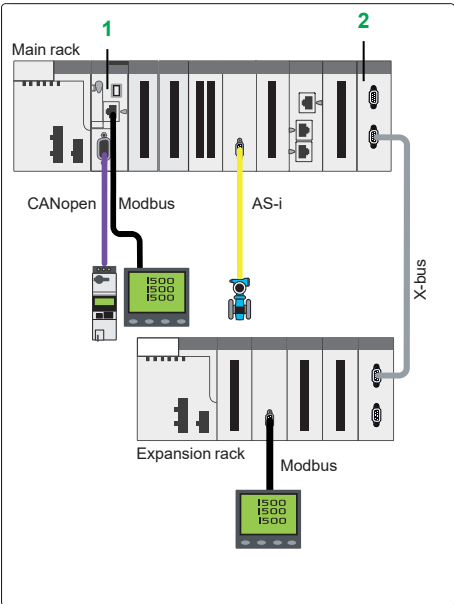
Integrated fieldbus architecture
