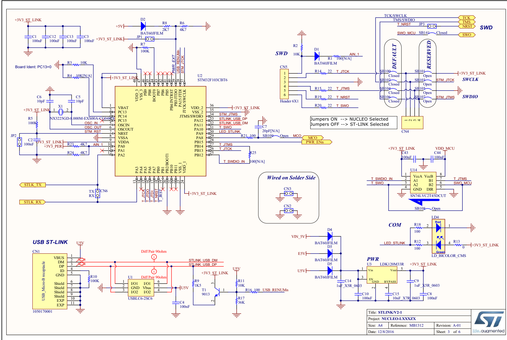
Figure 15. ST-LINK/V2-1
