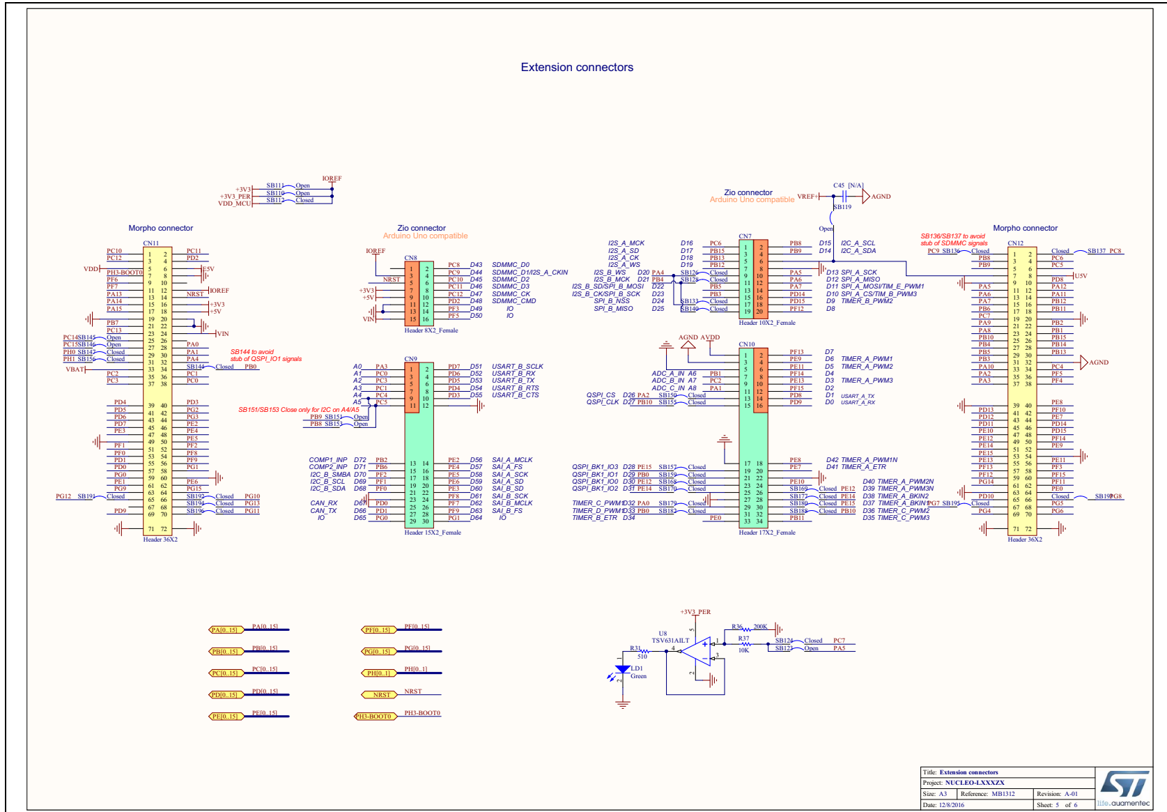
Figure 17. Extension connectors
