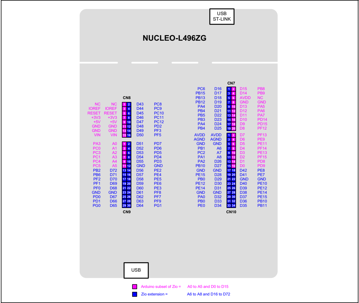
Figure 11. NUCLEO-L496ZG
