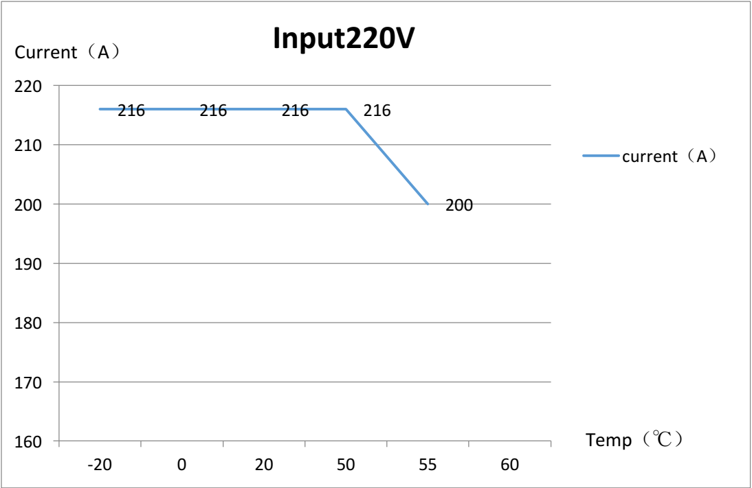
Max Load vs. Ambient Temperature Graph (220V input)
