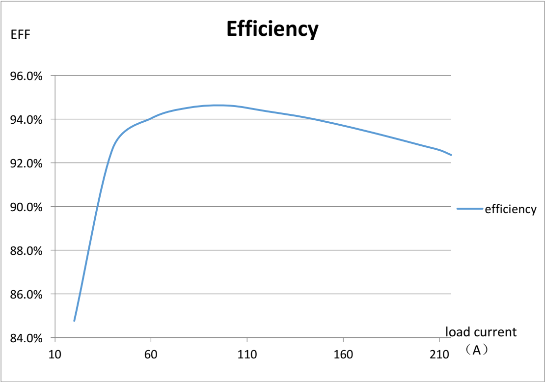
Efficiency vs Load (220V input)
