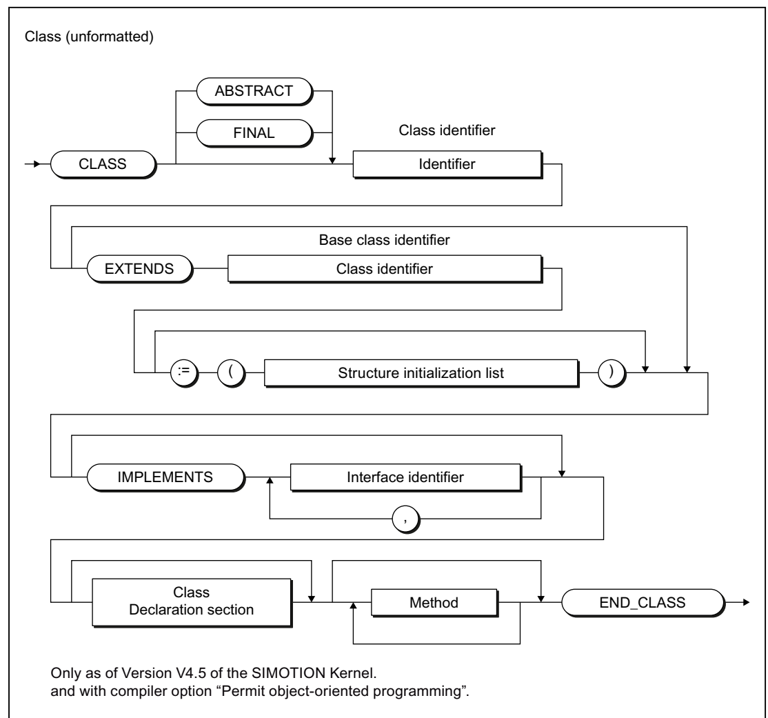
Figure 6-10 Syntax: Class
