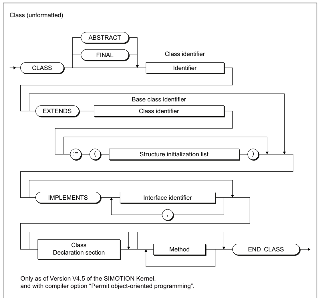
Figure 6-13 Syntax: Class
