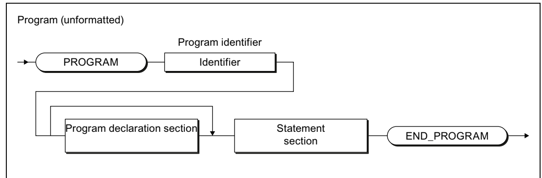
Figure 5-16 Syntax: Program
