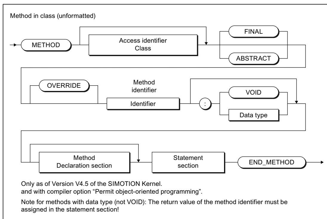
Figure A-37 Syntax: Method
