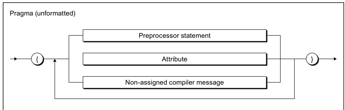
Figure 7-13 Syntax: Pragma
