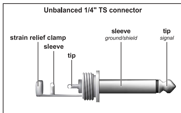
Fig. 4.2: 1/4" mono plug
