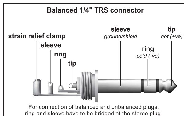
Fig. 4.3: 1/4" stereo plug
