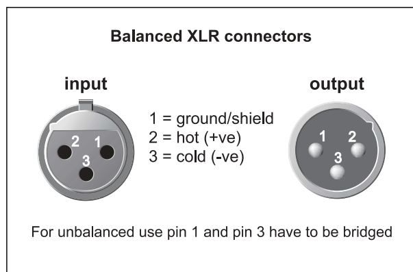
Fig. 4.1: XLR connections
