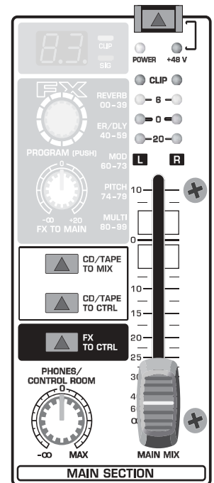
Fig. 2.4: Control elements of the main section
