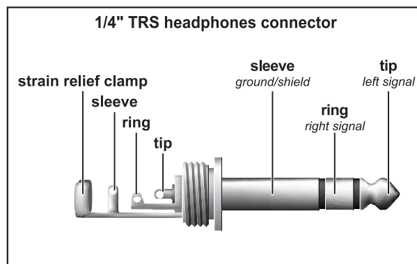
Fig. 4.4: Stereo plug for headphones connection
