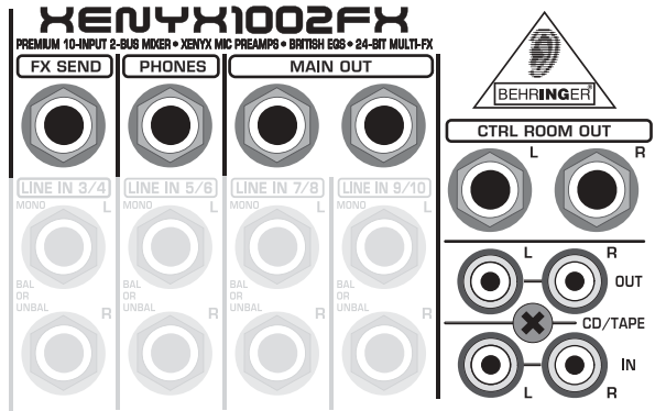
Fig. 2.3: Connectors of the main section
