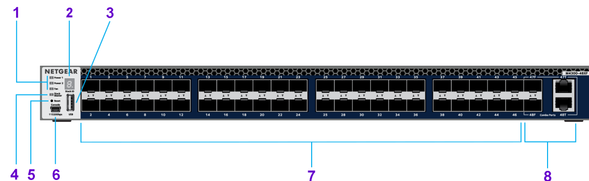
Figure 18. Front panel model M4300-48XF
