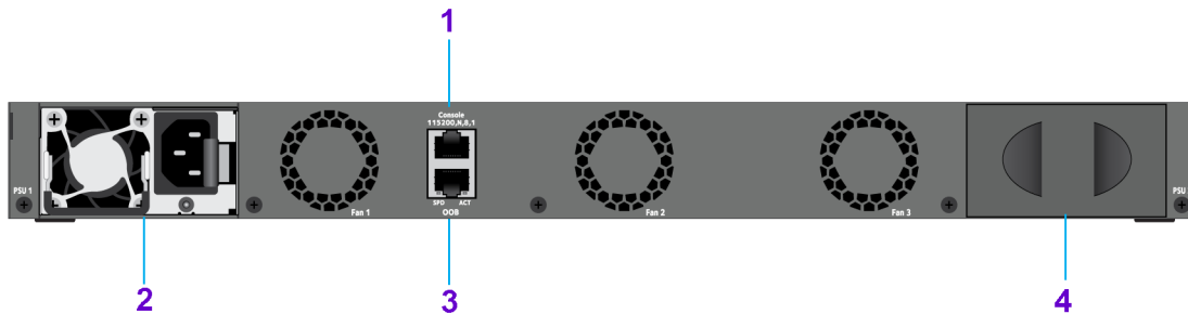
Figure 22. Back panel model M4300-48XF
