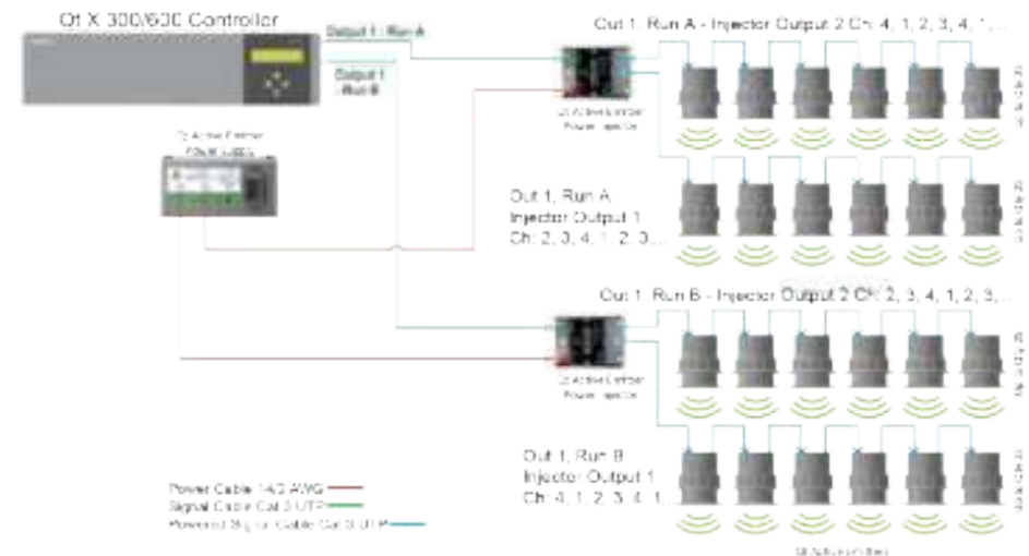
Figure 20. Active emitter runs and channel designations
