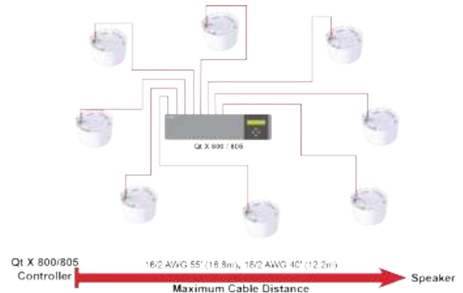
Figure 25. Speaker output connectors - maximum cable length
