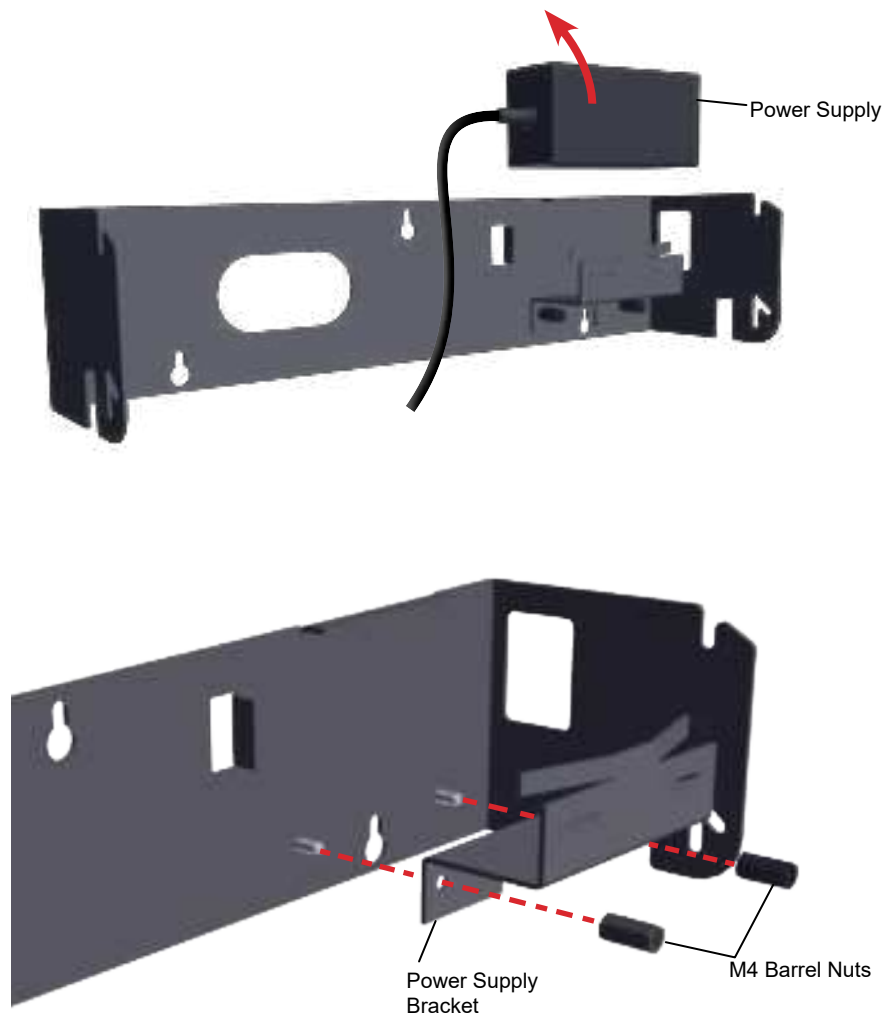
Figure 28. Remove power supply and bracket
