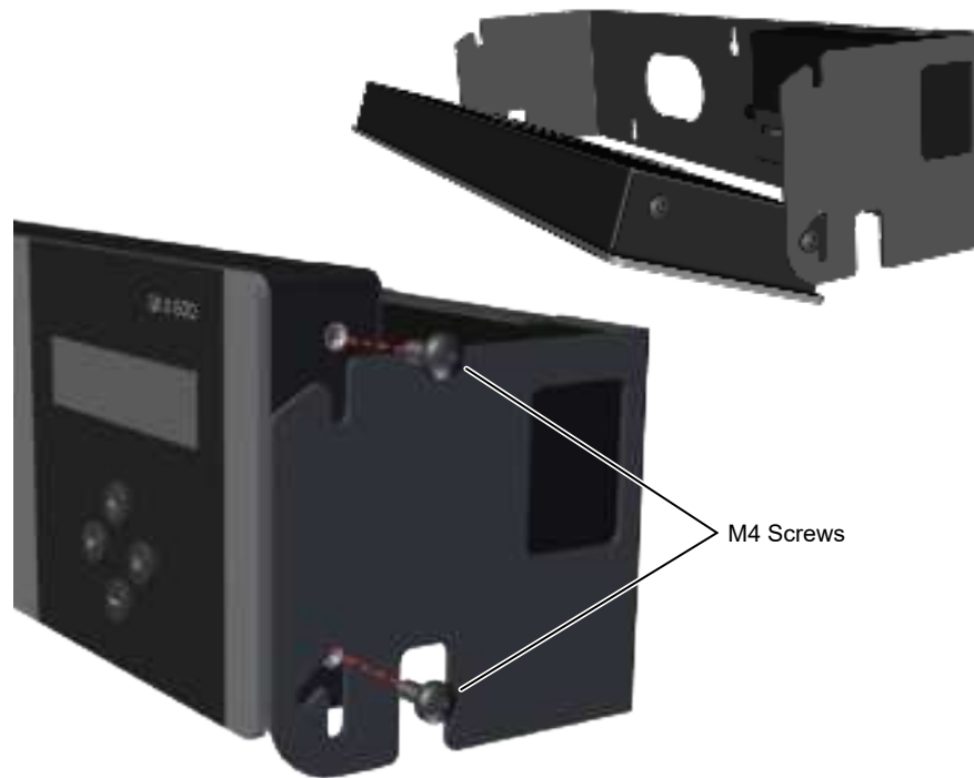
Figure 35. Mount unit to wall bracket and rotate down
