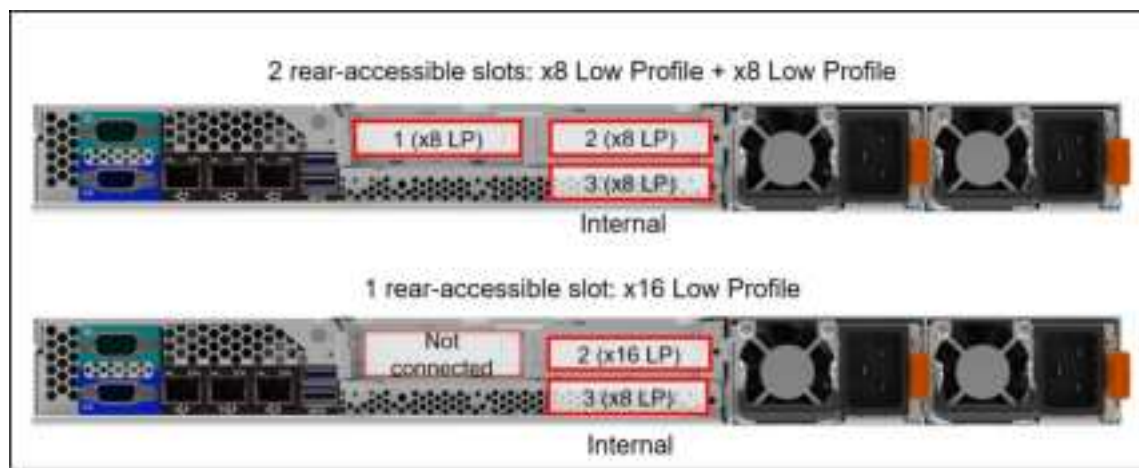
Figure 10. Slot locations
