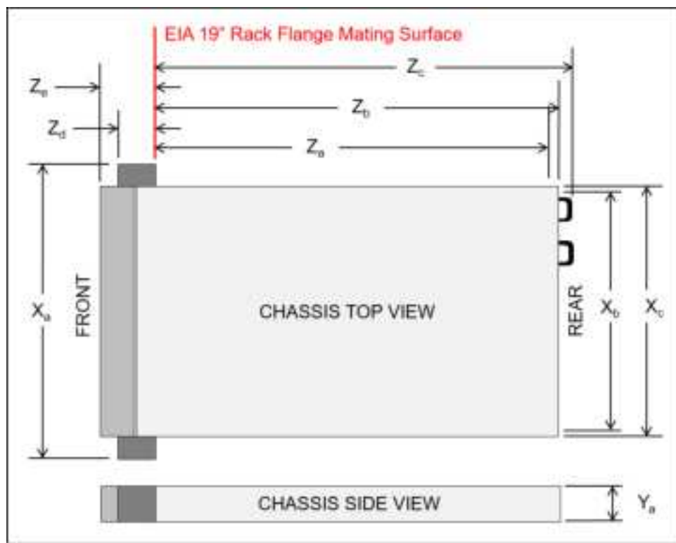
Figure 12. Server dimensions
