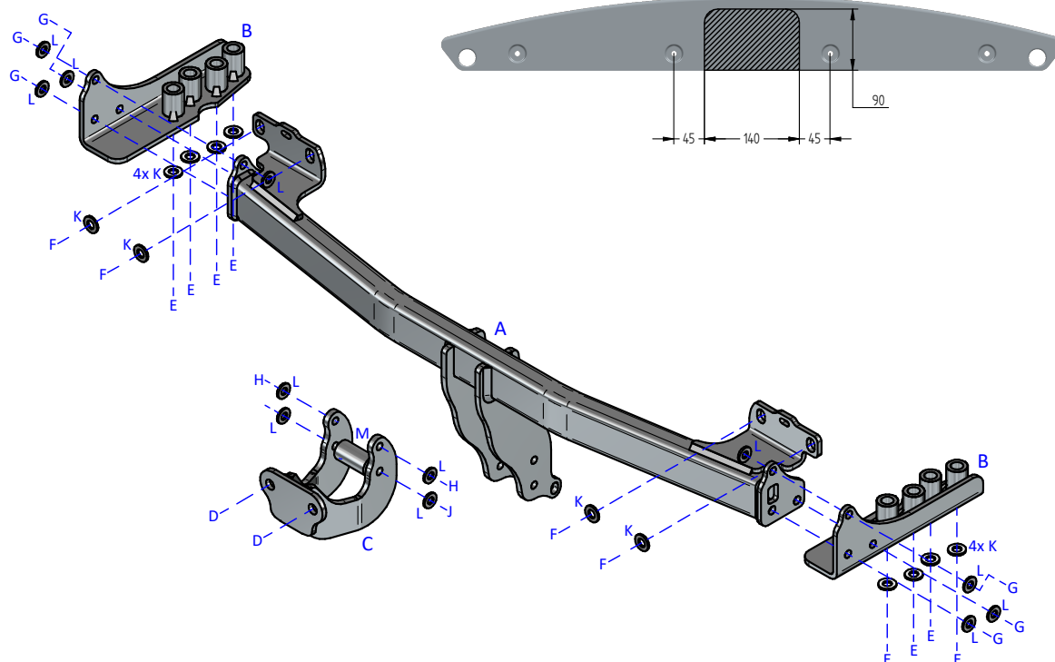
Bumper Cut Details Below
