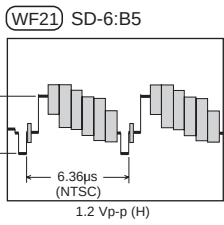
Composite waveform
