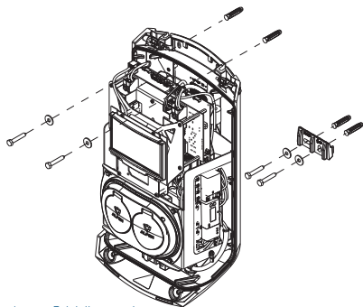
Image 3: Wall mounting
