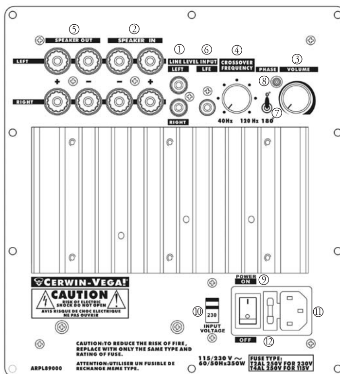
Figure 1. Connection panel for the Classic Series Subwoofers.
