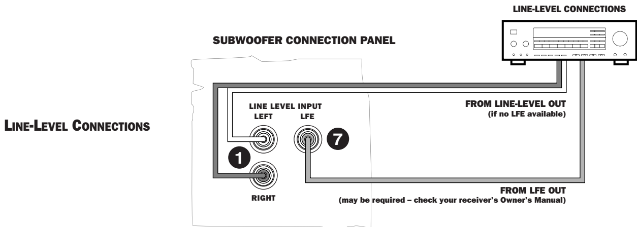
Figure 2. Connecting left and right line-level outputs of an A/V receiver to left and right line-level inputs of the Cerwin-Vega subwoofer. Remember to maintain left to left, right to right, (+) to (+) and (-) to (-) connections!
