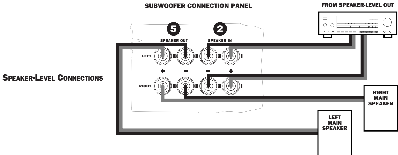
Figure 4. Connecting left and right speaker-level outputs of an A/V receiver to left and right speaker-level inputs of the subwoofer. Then connect left and right speaker-level outputs of the subwoofer, with the main left and right speakers of your system. Remember to maintain left to left, right to right, (+) to (+) and (-) to (-) connections.
