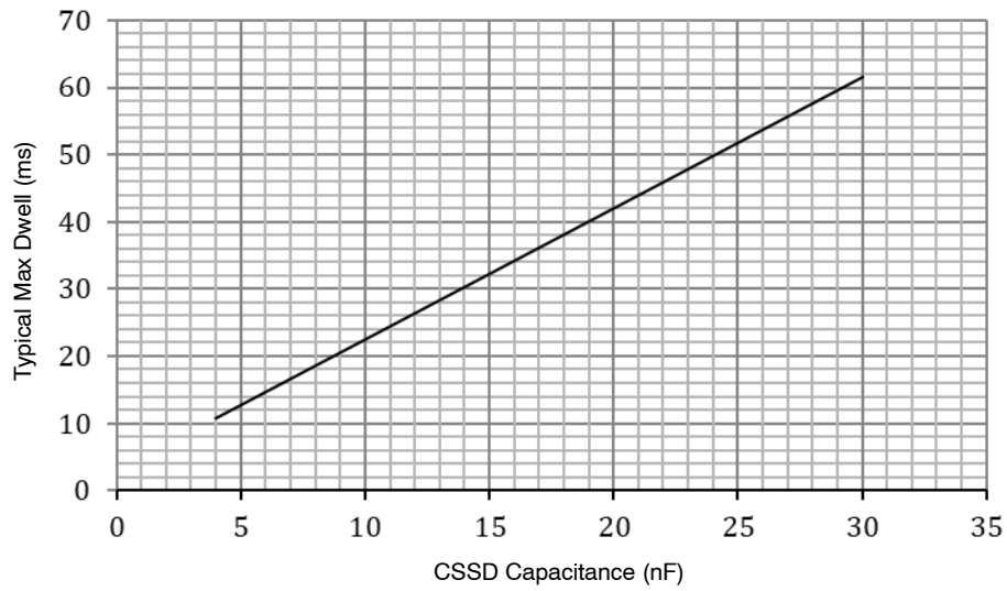
Figure 5. T_{D\text{MAX}} as Function of External CSSD Capacitor
