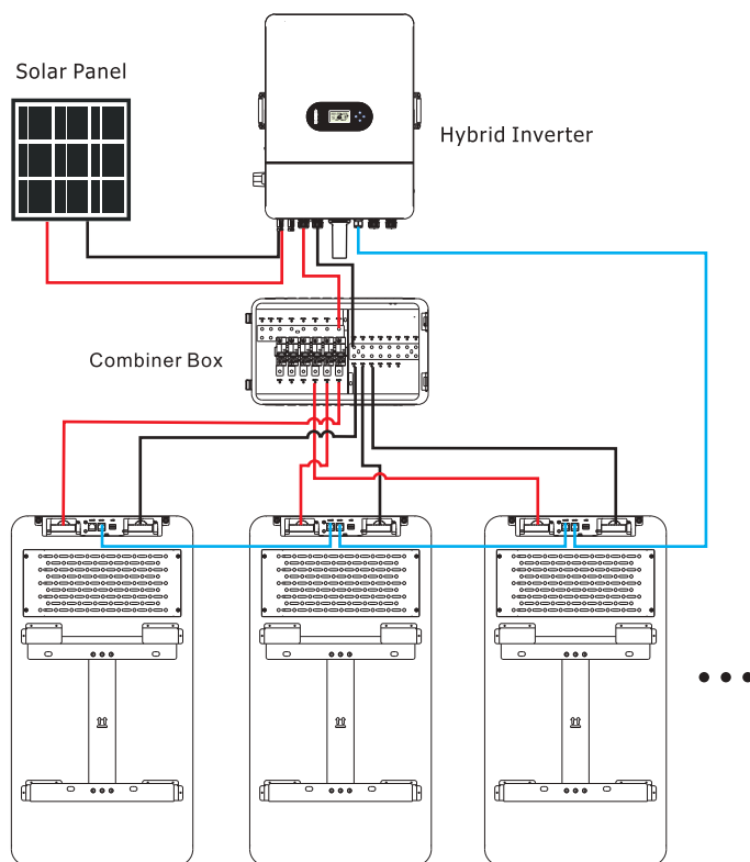
Figure 3-2 Multiple Battery Parallel System Connection Diagram
