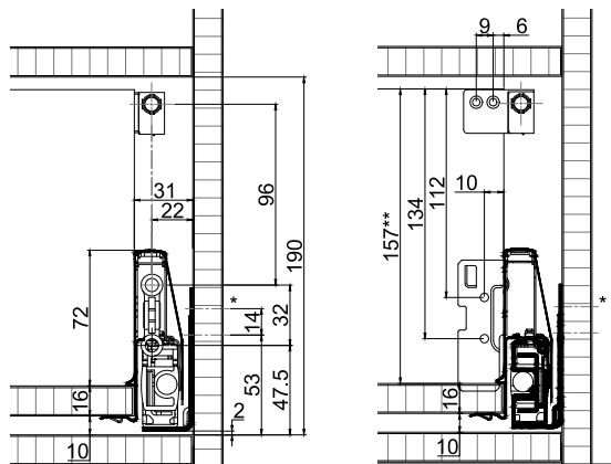
Front, screw-on
