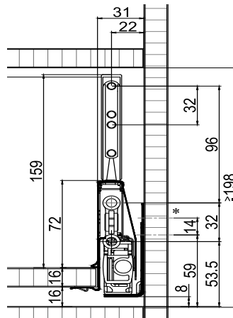
Front, screw-on
