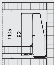
Soft-Close
