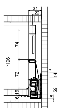
Front, screw-on
