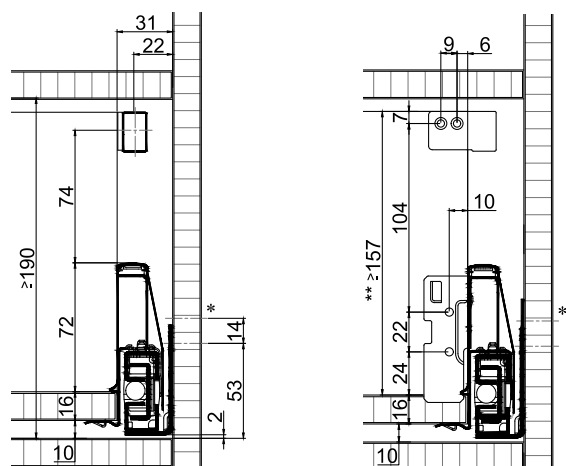
Front, screw-on
