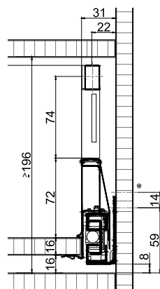
Front, screw-on
