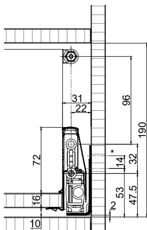
Front, screw-on
