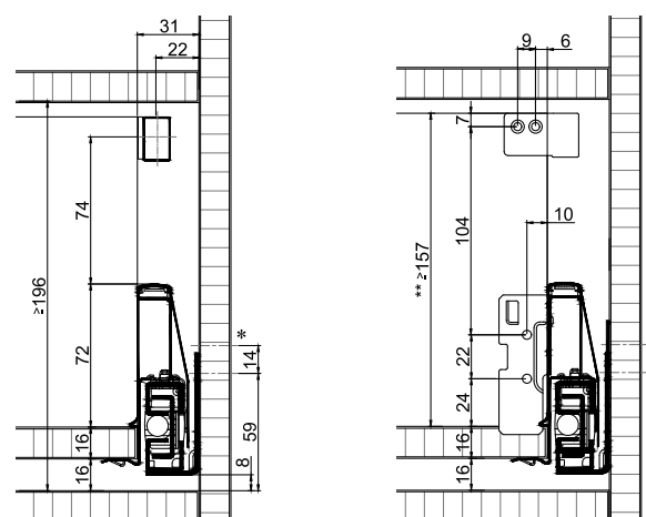
Front, screw-on
