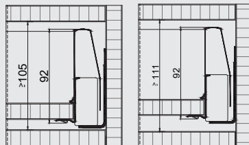
Soft-Close
