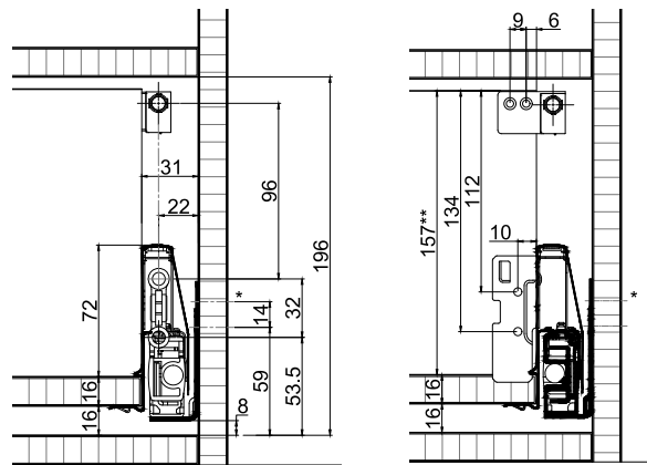
Front, screw-on
