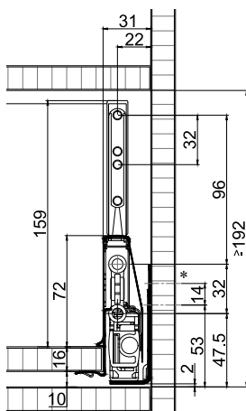
Front, screw-on
