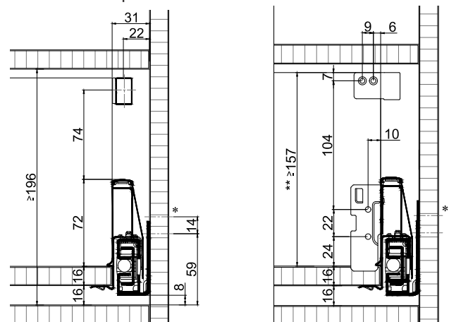
Front, screw-on
