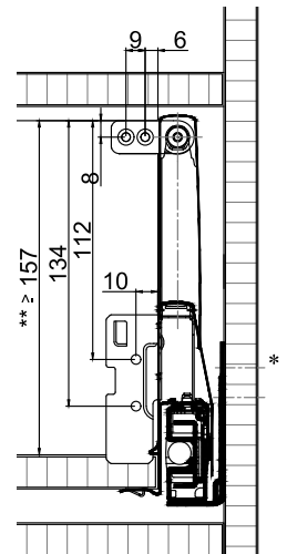
Back
