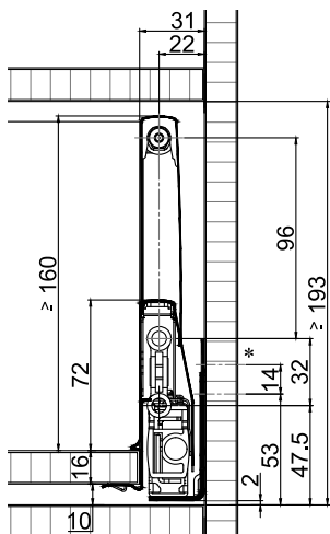
Front, screw-on
