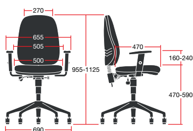
TEP/1D: Overall Dimensions: 690w x 690d x 1125h
