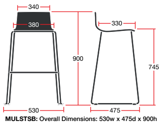
MULSTSB: Overall Dimensions: 530w x 475d x 900h
