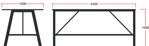
AB24/12: Overall Dimensions: 2400w x 1200d x 1050h
