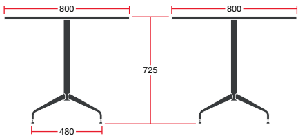
MT12/CIR08: Overall Dimensions: 800w x 800d x 725h
