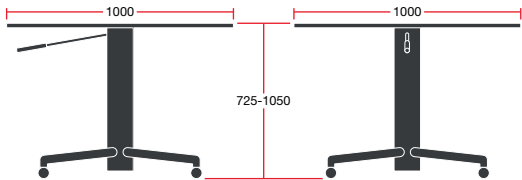
MT10HA/CIR10: Overall Dimensions: 1000w x 1000d x 1050h
