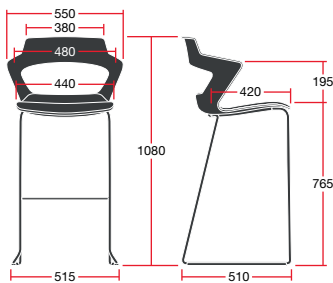
ZENSTSBUS: Overall Dimensions: 550w x 520d x 1080h
