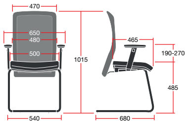
MERC/4D: Overall Dimensions: 650w x 680d x 1015h
