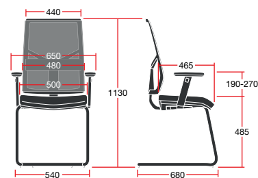
MIXC/4D: Overall Dimensions: 650w x 680d x 1130h
