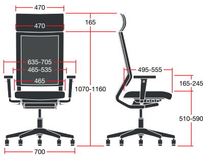
ISITML/MH/4DL: Overall Dimensions: 705w x 700d x 1325h
