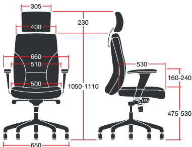
OPU: Overall Dimensions: 650w x 750d x 1340h
