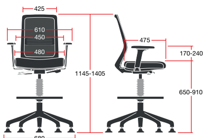
VIDD/1D: Overall Dimensions: 680w x 680d x 1405h
