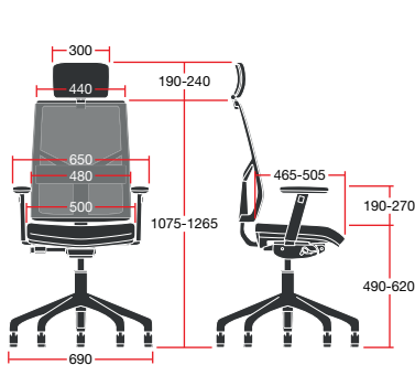
MIX/4D/UH: Overall Dimensions: 690w x 690d x 1505h
