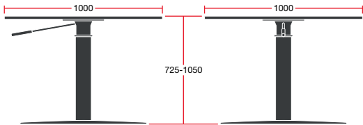
MT09HA/CIR10: Overall Dimensions: 1000w x 1000d x 1050h
