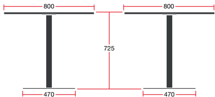
MT07/CIR08: Overall Dimensions: 800w x 800d x 725h
