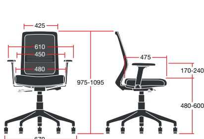
VID/1D: Overall Dimensions: 670w x 670d x 1095h
