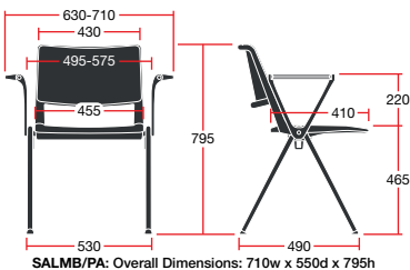
SALMB/PA: Overall Dimensions: 710w x 550d x 795h
