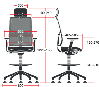
MIXD/4D/UH: Overall Dimensions: 690w x 690d x 1795h
