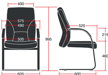
OPUC: Overall Dimensions: 605w x 670d x 995h
