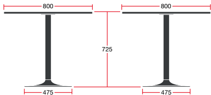
MT06/CIR08: Overall Dimensions: 800w x 800d x 725h
