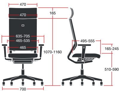
ISITLI/UH/4DL: Overall Dimensions: 705w x 700d x 1325h
