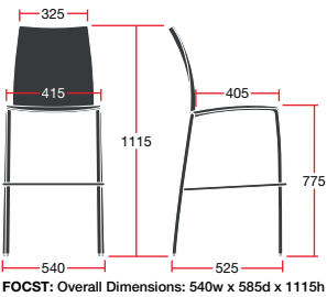
FOCST: Overall Dimensions: 540w x 585d x 1115h
