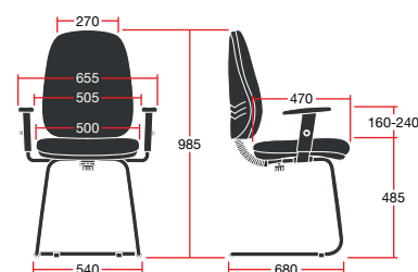
TEPC/1D: Overall Dimensions: 655w x 680d x 985h
