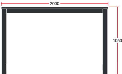
KITHB20/9: Overall Dimensions: 2000w x 900d x 1050h
