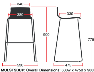
MULSTSBUP: Overall Dimensions: 530w x 475d x 900h
