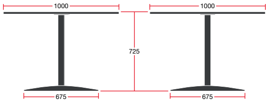
MT04/SQR10: Overall Dimensions: 1000w x 1000d x 725h
