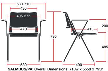
SALMBUS/PA: Overall Dimensions: 710w x 555d x 795h
