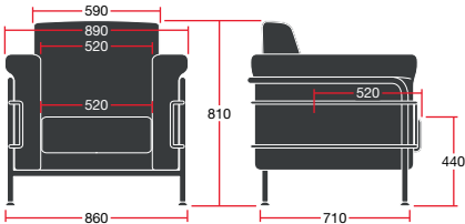
NAP1: Overall Dimensions: 890w x 780d x 810h
