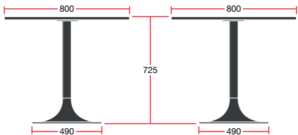
MT05/SQR08: Overall Dimensions: 800w x 800d x 725h
