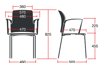
LLGPSPB/GLA: Overall Dimensions: 570w x 535d x 825h
