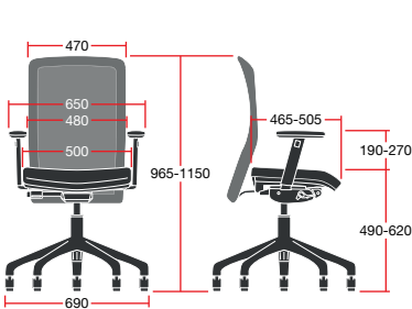
MER/4D: Overall Dimensions: 690w x 690d x 1150h
