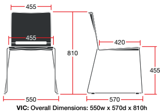
VIC: Overall Dimensions: 550w x 570d x 810h
