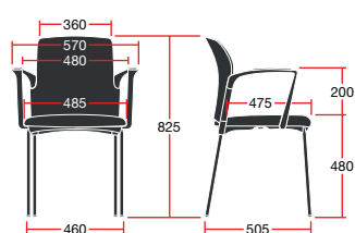
LLGUSPB/GLA: Overall Dimensions: 570w x 535d x 825h
