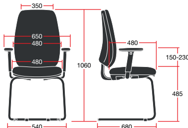
LORC/U/3D: Overall Dimensions: 650w x 680d x 1060h
