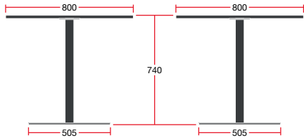
MT01/CIR08: Overall Dimensions: 800w x 800d x 740h
