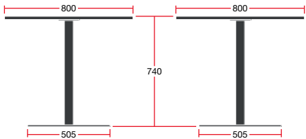
MT01/SQR08: Overall Dimensions: 800w x 800d x 740h
