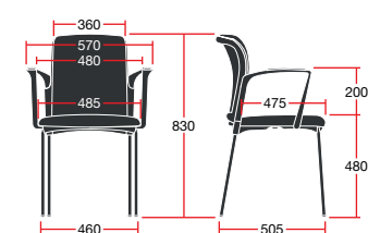
LLGUSUB/GLA: Overall Dimensions: 570w x 535d x 830h
