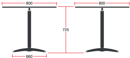
MT11/CIR08: Overall Dimensions: 800w x 800d x 725h
