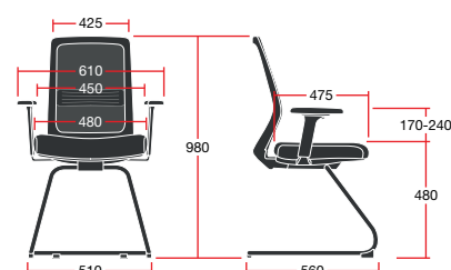
VIDC/1D: Overall Dimensions: 510w x 560d x 980h
