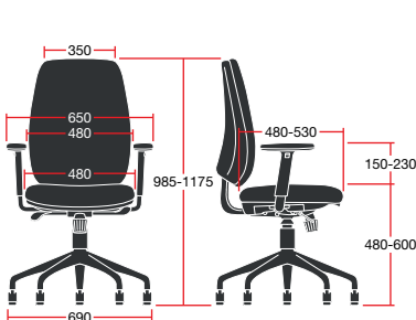
LOR/U/3D: Overall Dimensions: 690w x 690d x 1175h
