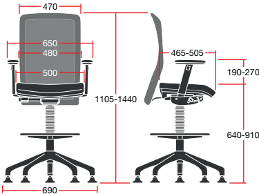
MERD/4D: Overall Dimensions: 690w x 690d x 1440h
