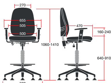
TEPD/1D: Overall Dimensions: 690w x 690d x 1410h
