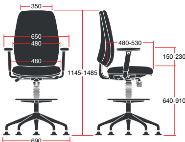
LORD/U/3D: Overall Dimensions: 690w x 690d x 1485h
