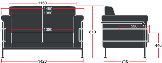
NAP2: Overall Dimensions: 1450w x 780d x 810h
