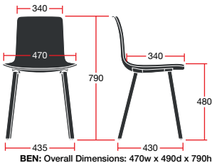
BEN: Overall Dimensions: 470w x 490d x 790h
