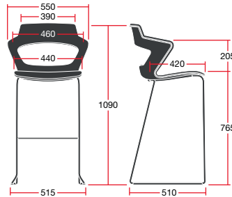
ZENSTSBUSUB: Overall Dimensions: 550w x 520d x 1090h
