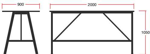
HB20/9: Overall Dimensions: 2000w x 900d x 1050h
