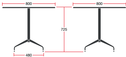
MT12/SQR08: Overall Dimensions: 800w x 800d x 725h
