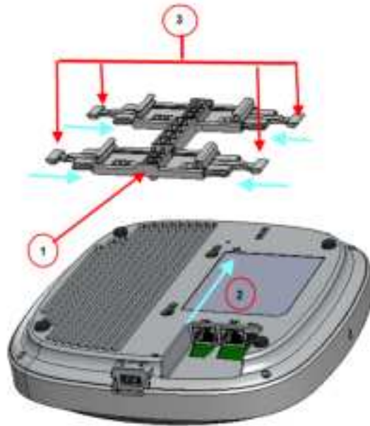
FIGURE 7 Attaching the T-bar Bracket to the AP
