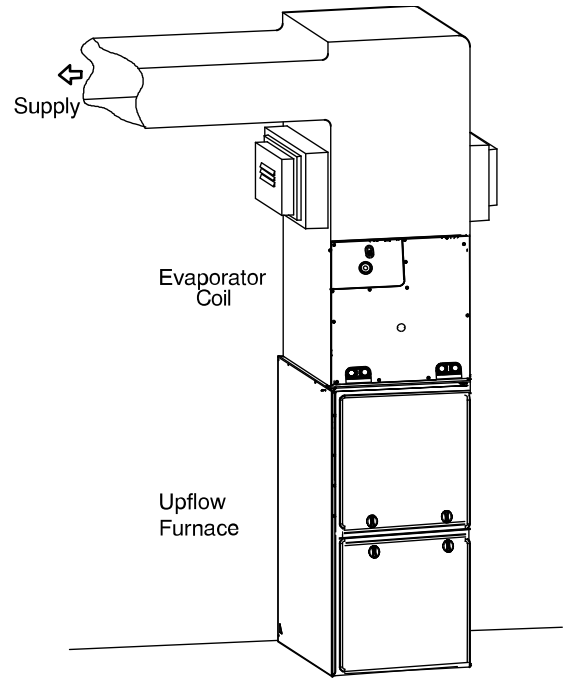
Fig. 10 – Humidifier Application
