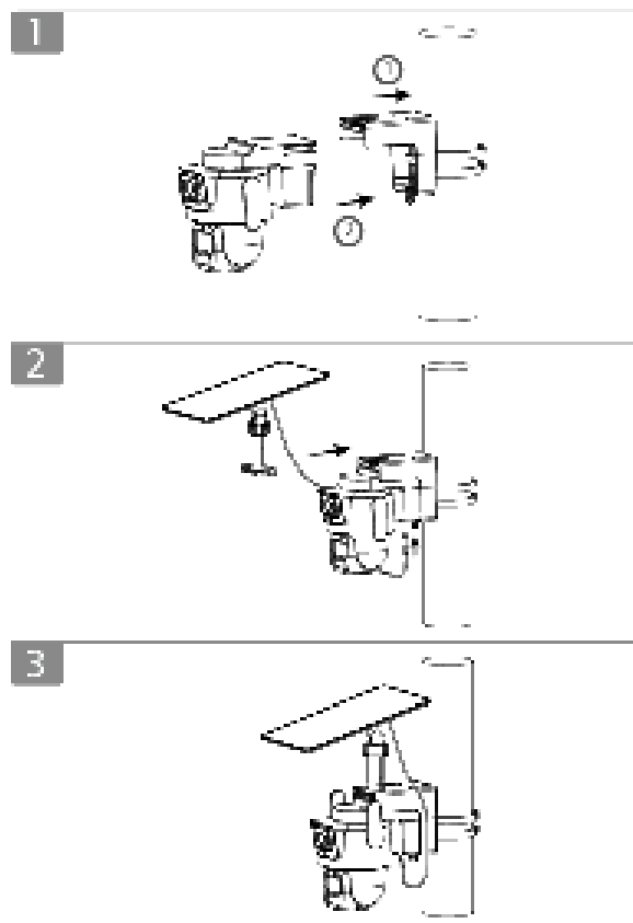
Figure 4-6 Pole mount installation
