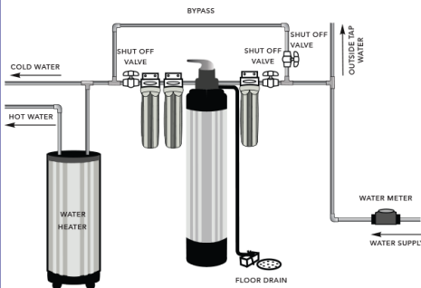
Mechanical System/Polyglass Water Filter System
