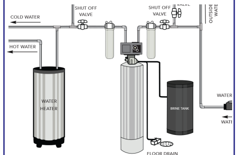
Softener, Tannin or Nitrate System/ Stainless Steel Water Filter System
