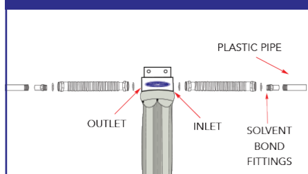
Connecting to plastic pipe
