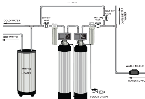
Automatic System/Polyglass Water Filter System
