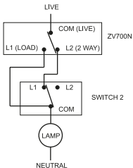
3 WIRE SYSTEM AFTER
