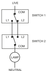
3 WIRE SYSTEM BEFORE
