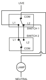
5+3 WIRE SYSTEM BEFORE
