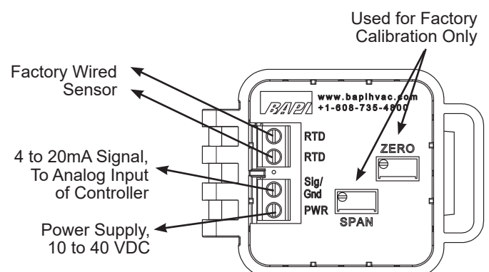
Fig. 4: Transmitter with Terminals
