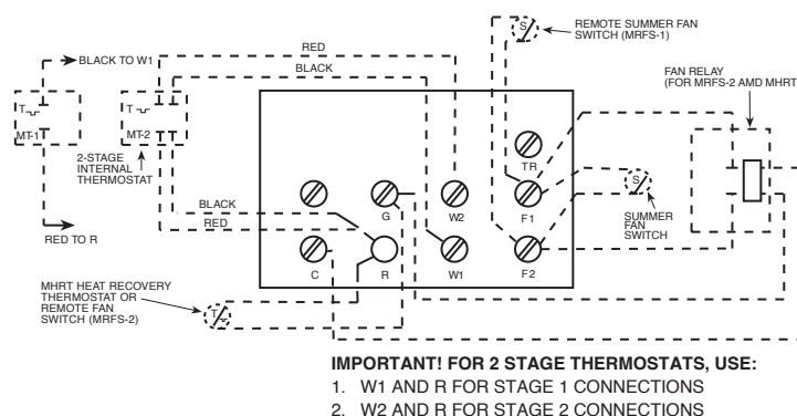
Figure 5. Control Terminal Board (for Heaters With Contactors)
