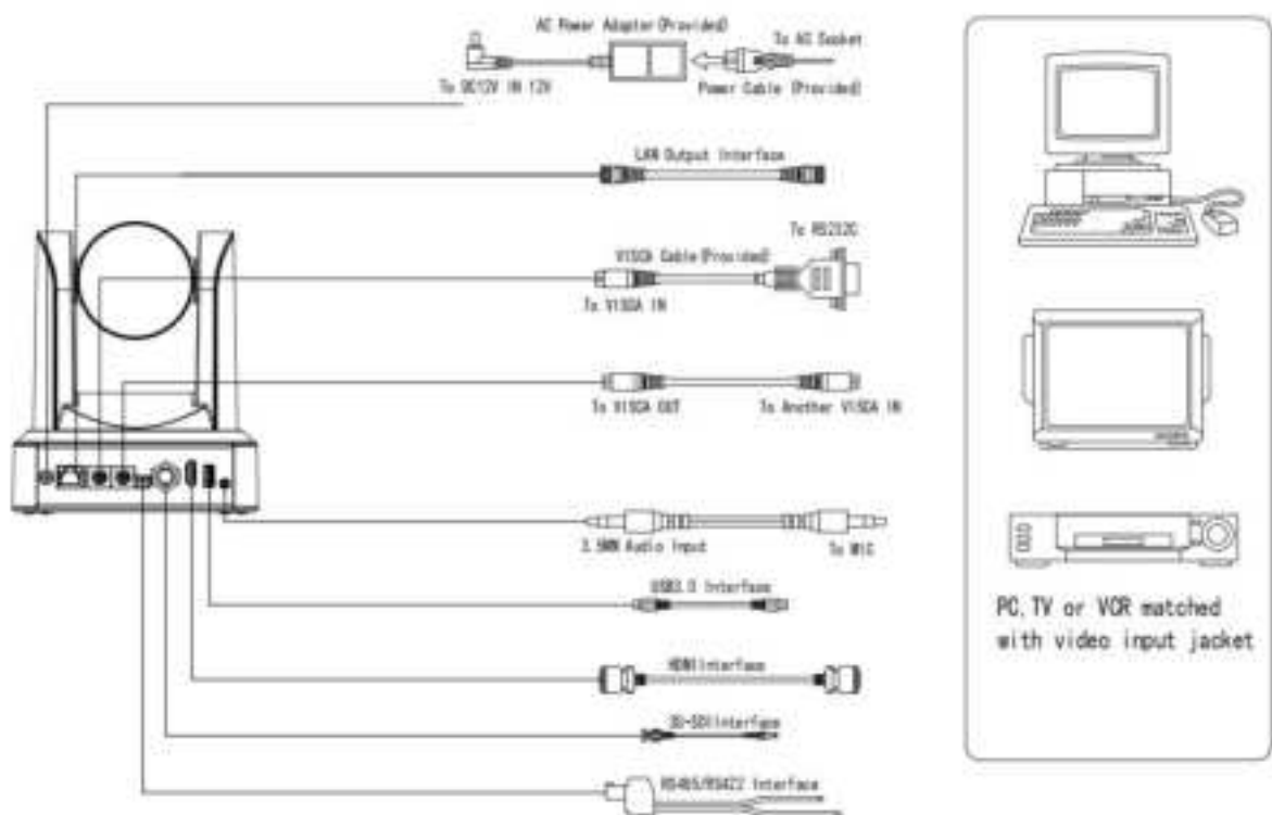
Figure 2-2 Back Panel Image
