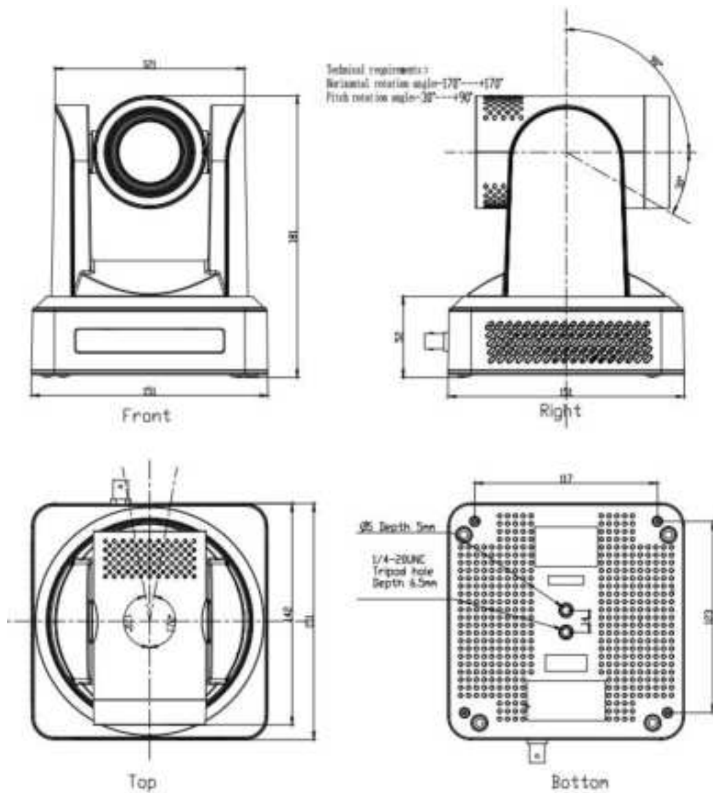
Figure2-1 Dimension
