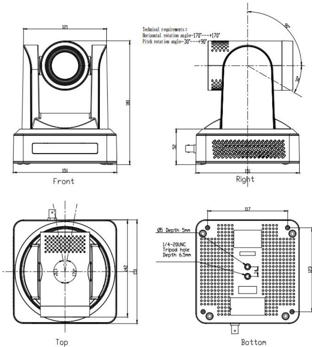
Figure2-1 Dimension
