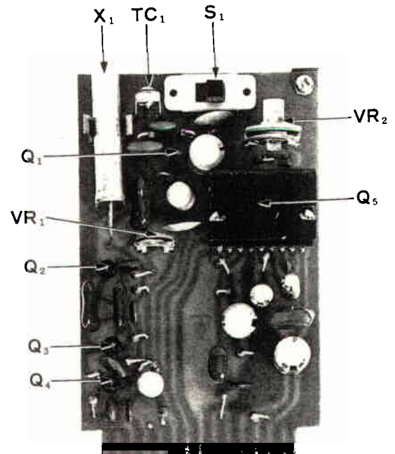
Fig. 16 AF-CALIB UNIT
