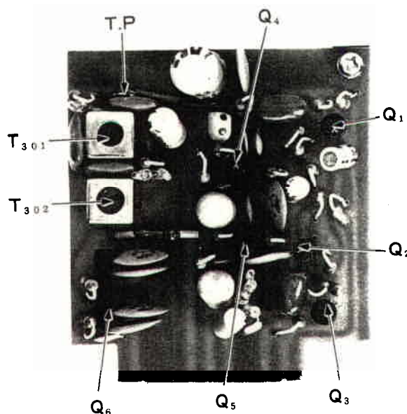
Fig. 22 FM UNIT
