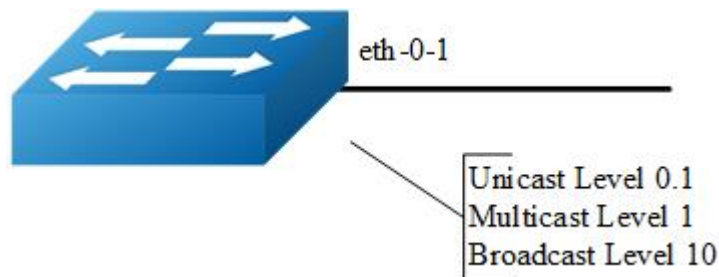
Percentage Storm Control
