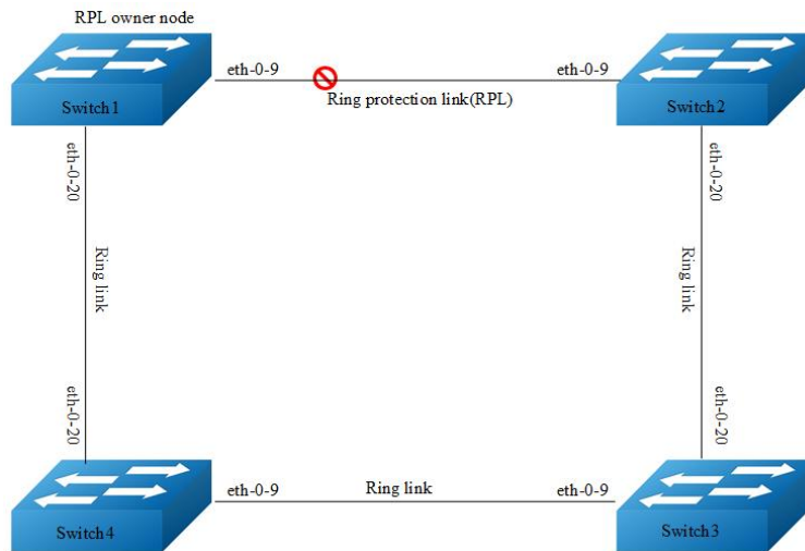
Topology of single G8032 ring
