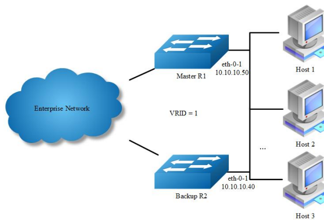
VRRP with one virtual router
