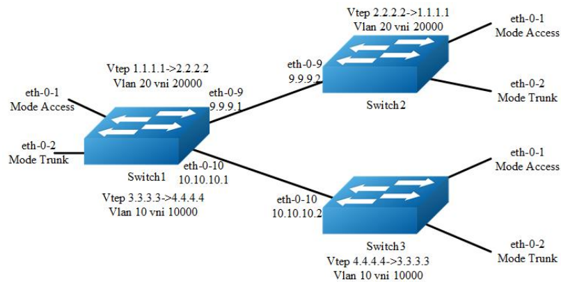
Overlay multiple source ip
