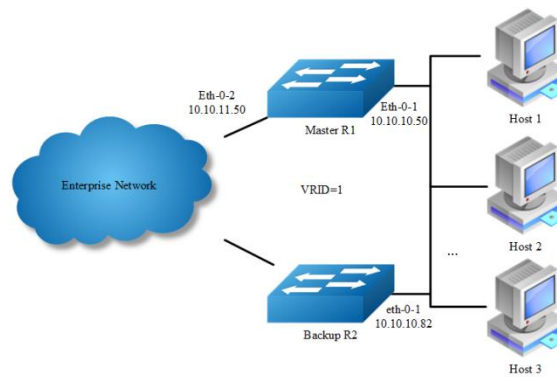
VRRP Circuit Failover
