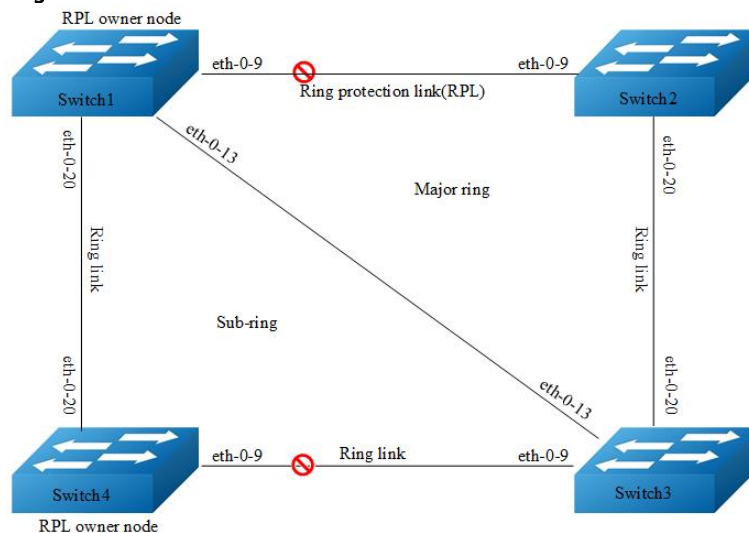
Topology of multiple G8032 rings
