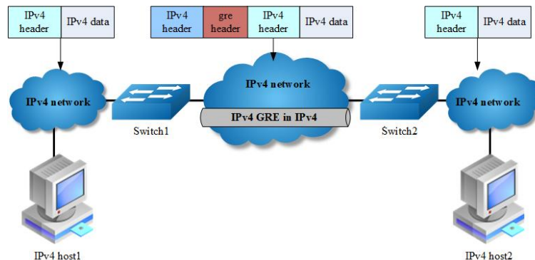
IPv4 gre over IPv4
