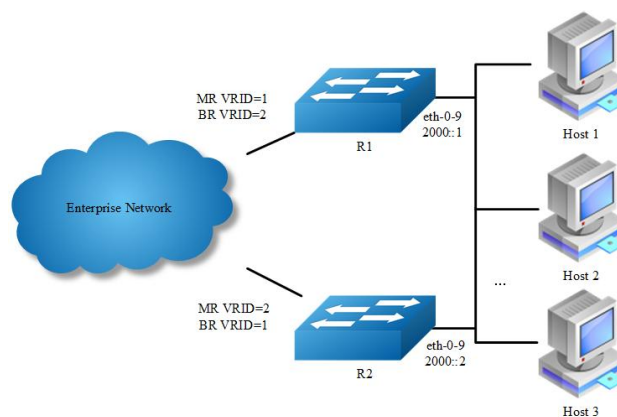
IPv6 VRRP with two virtual router
