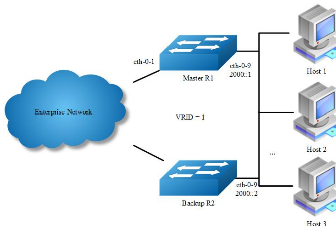
IPv6 VRRP Circuit Failover
