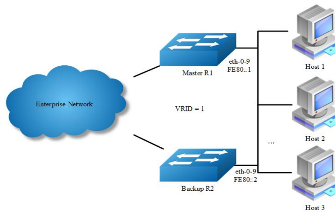
IPv6 VRRP with one virtual router
