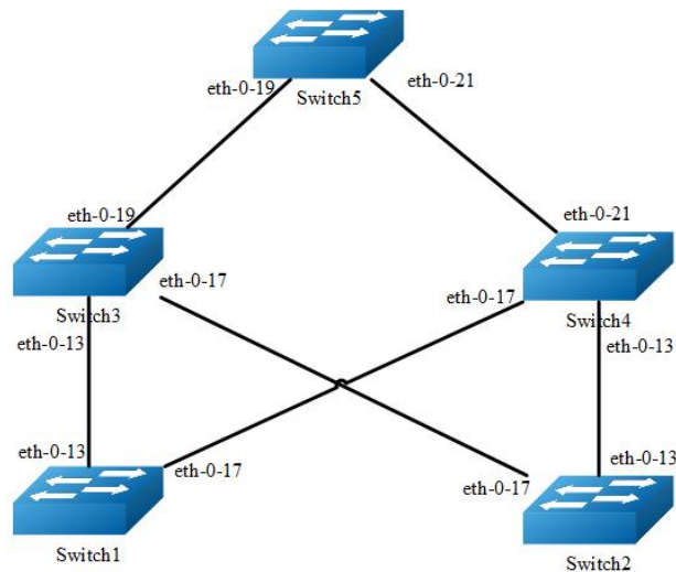
Smart-Link Typical Topology
