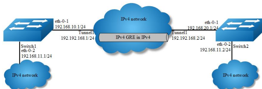
IPv4 gre Tunnel
