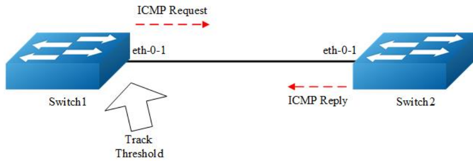
Track ip sla
