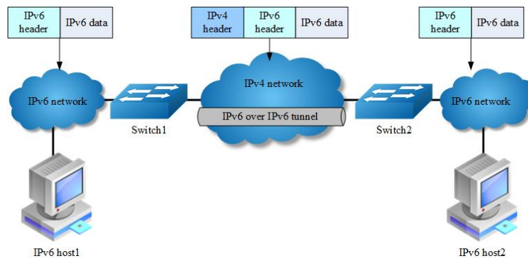
IPv6 over IPv4 Tunnel
