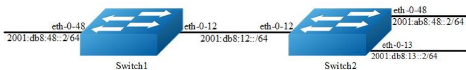
RIPng Route Distribute Filters
