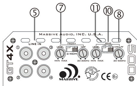
FIG 2. 4-CH AMPLIFIER PANEL LAYOUT GT4X
