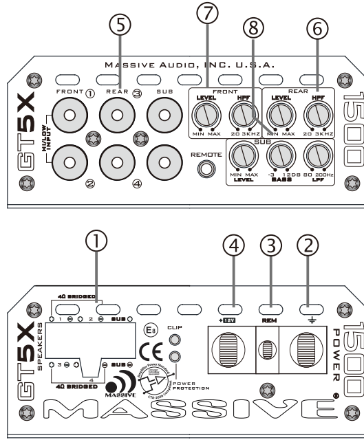
FIG 3. 5-CH AMOLIFIER PANEL LAYOUT GT5X
