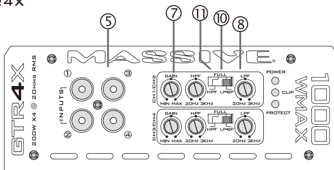
FIG 2. 4-CH AMPLIFIER PANEL LAYOUT GTR4X
