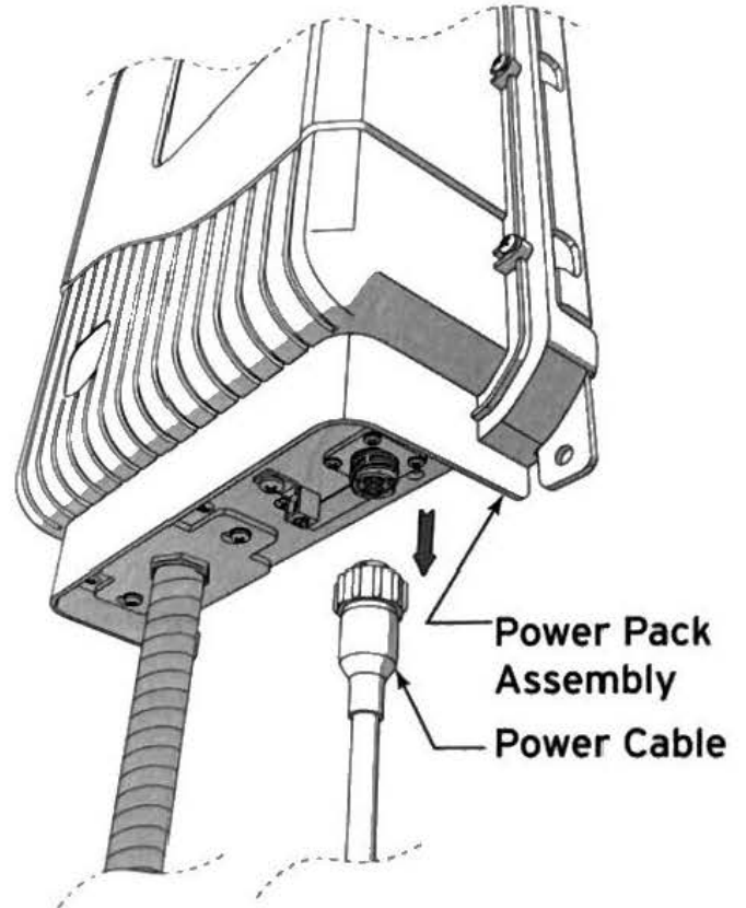
Figure 3. Disconnect Power
