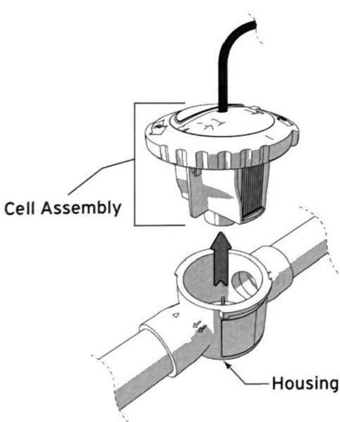
Figure 2. Remove Cell Assembly
