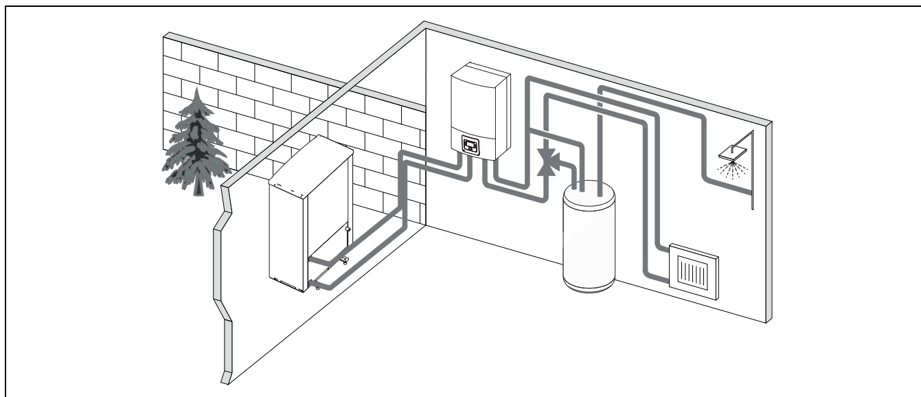
Fig. 3 Heat pump Compress 7001i/7400i AW, indoor unit AWE with electric booster heater and external hot water cylinder.
