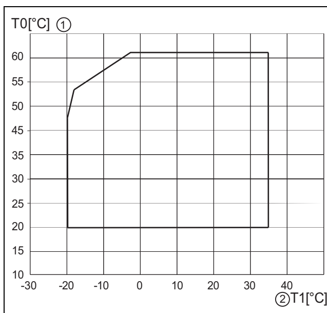
Fig. 1 Heat pump without auxiliary heater
