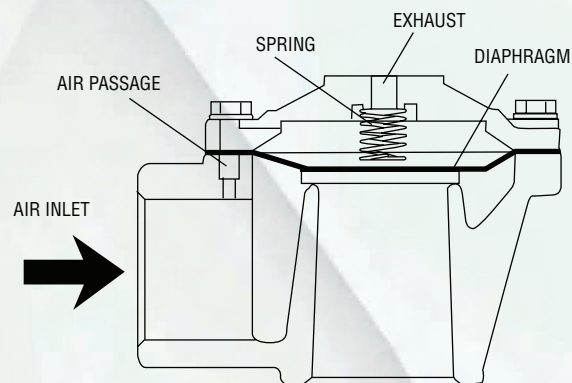
Figure 1. Closed Position
