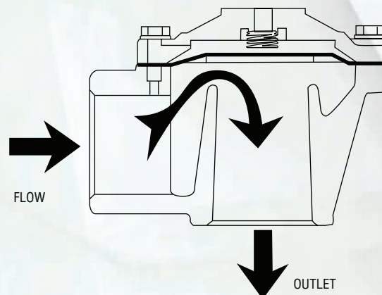
Figure 2. Open Position
