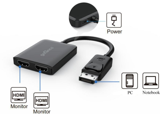
Figure 2: Connection Diagram
