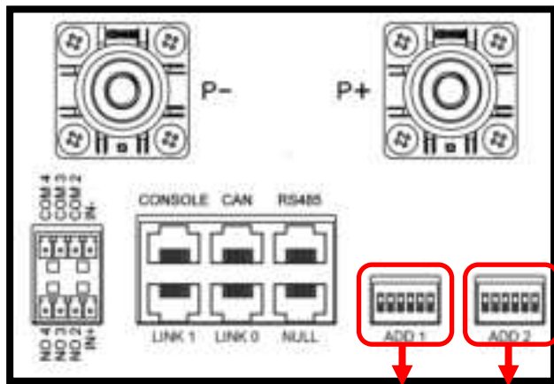
Pi LV1 BCU interface
