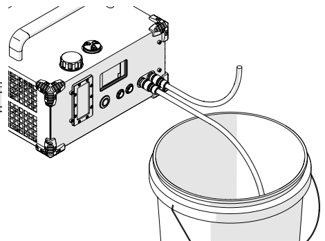
Fig. 9 - Draining coolant
