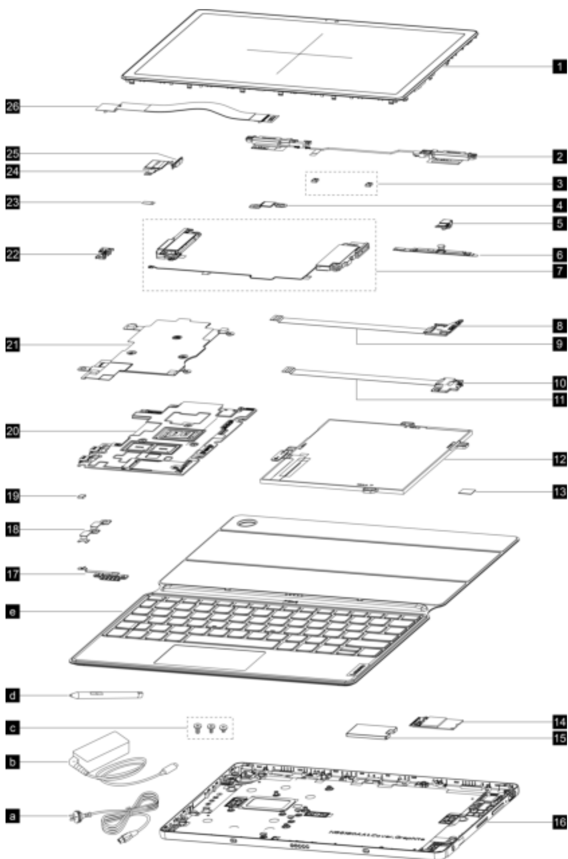
Figure 1. Exploded view
