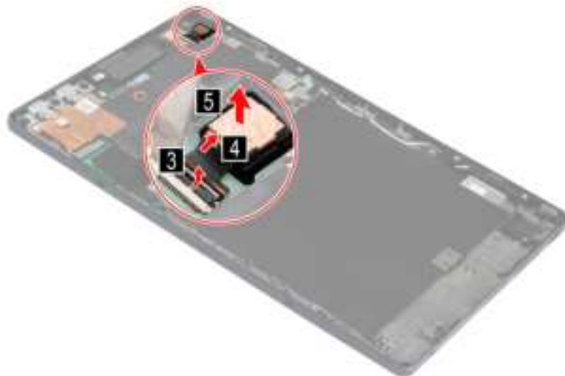
Figure 16. Remove the rear camera
