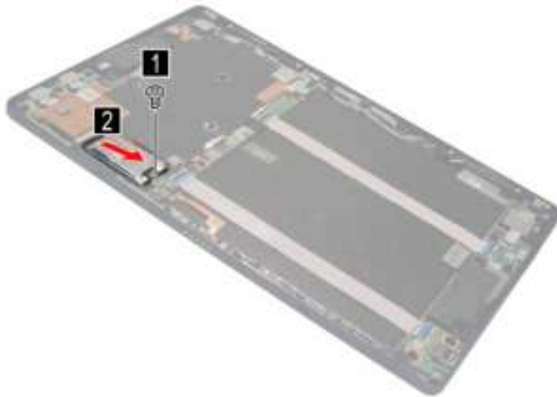
Figure 18. Remove one screw and the solid-state drive
