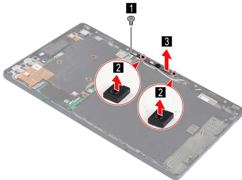
Figure 14. Pull the front cameras out of the LCD cover
