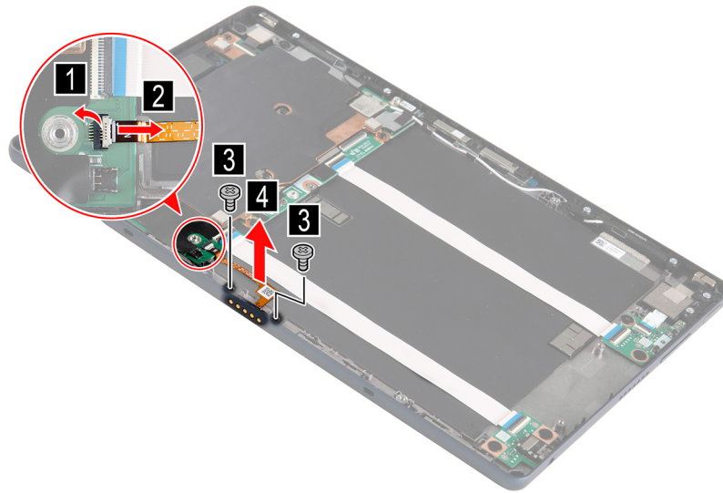
Figure 7. Disconnect the pogo pin cable from the system board, remove two screws and the pogo pin cable
