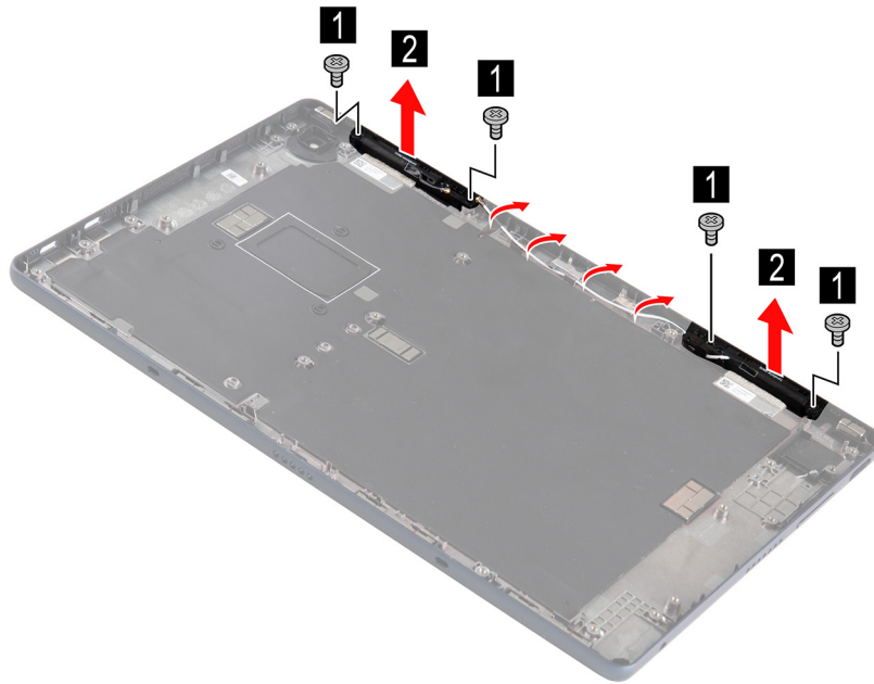
Figure 25. Remove four screws and the antennas
