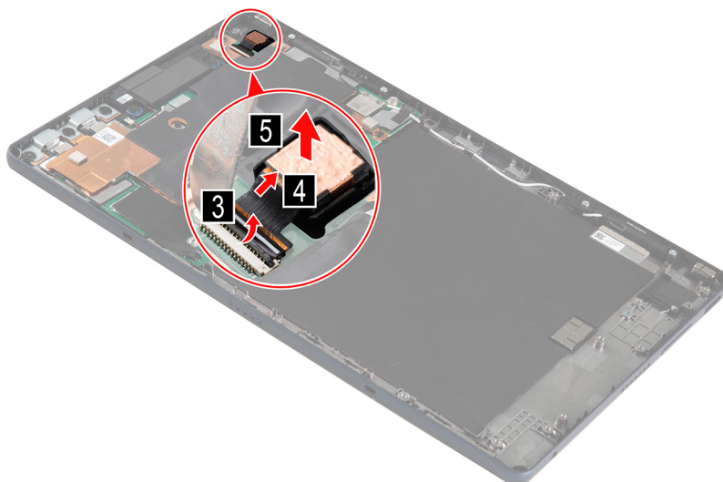
Figure 16. Remove the rear camera
