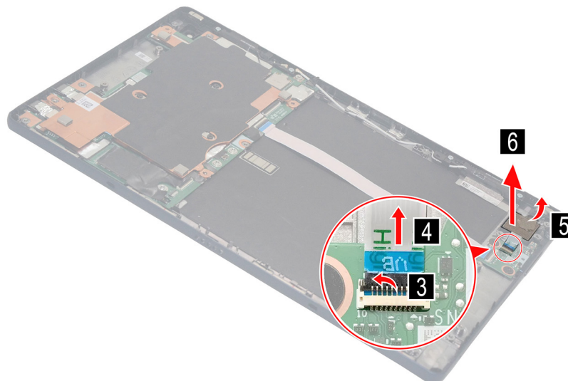
Figure 10. Disconnect the fingerprint board cable and then remove the fingerprint board
