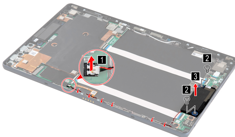
Figure 6. Disconnect the speaker cables, remove two screws and the speaker
