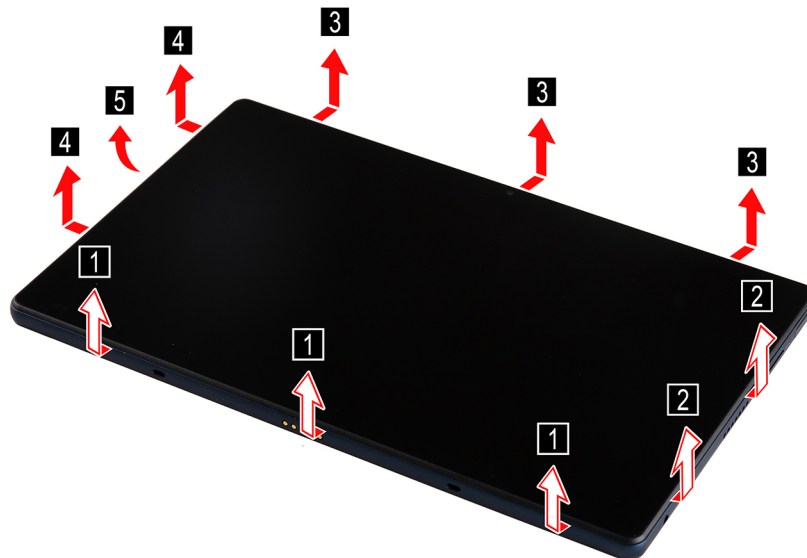
Figure 2. Pry up the latches and lift the LCD module
