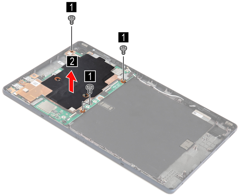
Figure 23. Remove three screws and remove the system board
