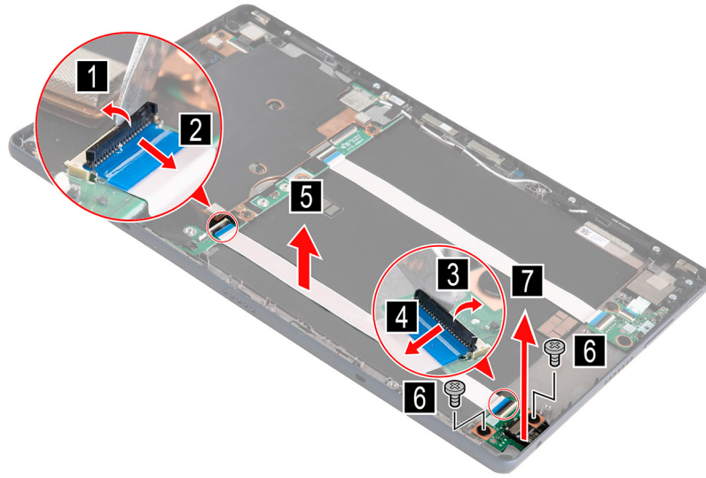
Figure 8. Remove two screws, disconnect the audio board cable and remove the audio board
