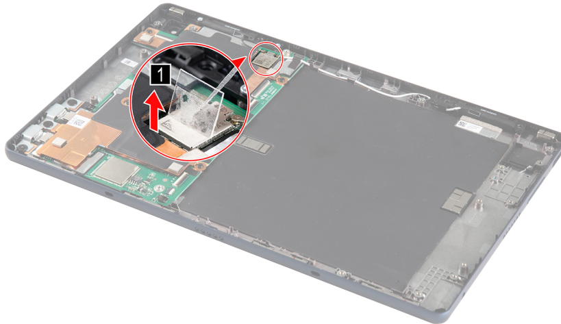
Figure 20. Remove the the WLAN mylar
