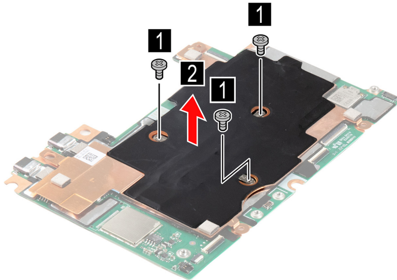
Figure 24. Remove three screws and the heat sink
