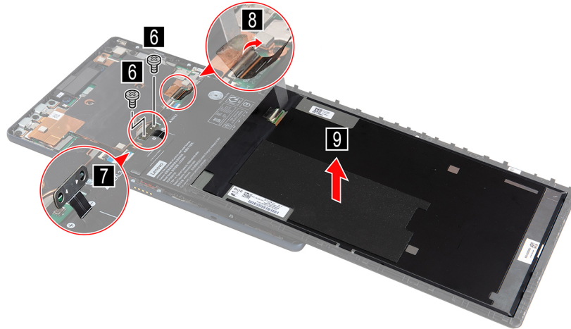
Figure 3. Remove two screws, disconnect the battery pack cable, remove the LCD cable protective mylar and the LCD module
