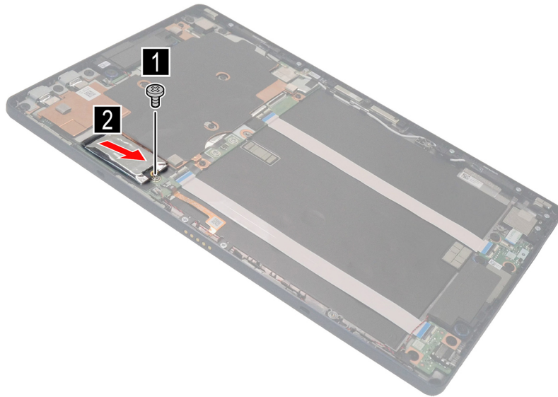
Figure 18. Remove one screw and the solid-state drive
