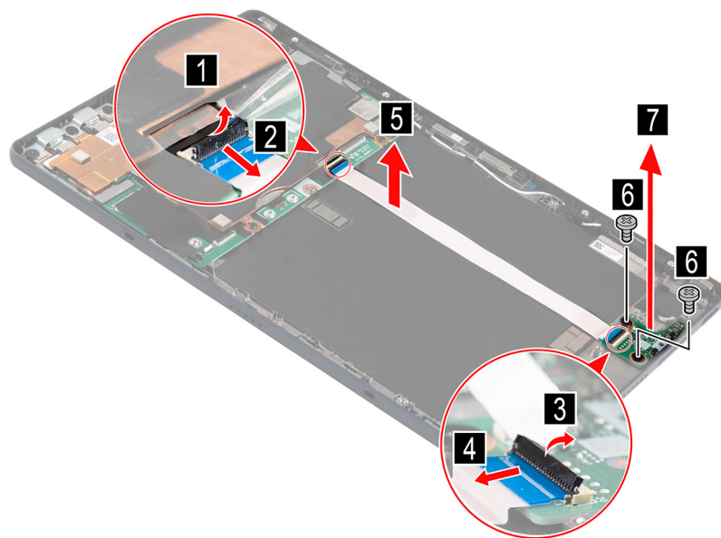
Figure 12. Remove two screws, disconnect the volume board and remove the volume board
