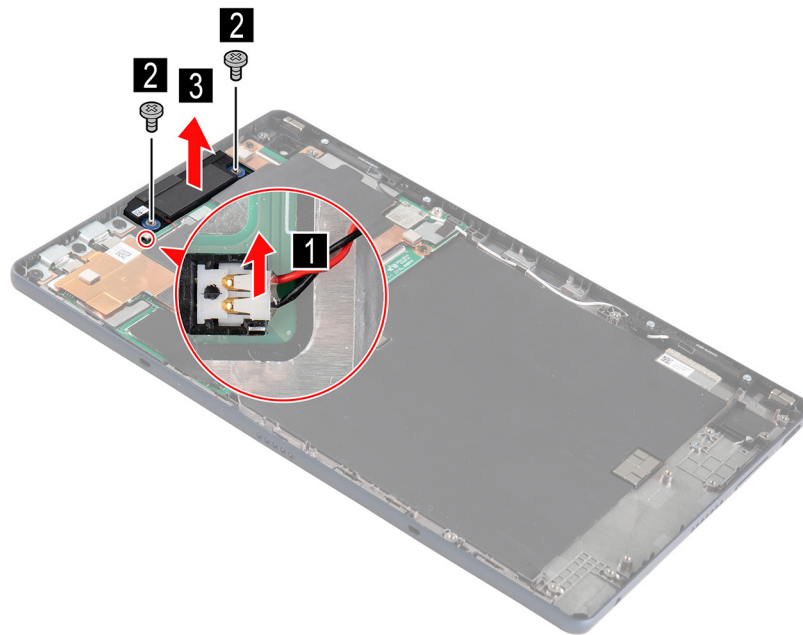
Figure 17. Disconnect the speaker cables, remove two screws and the speaker
