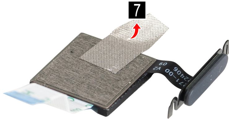
Figure 11. Remove the fingerprint conductive tape from the fingerprint board
