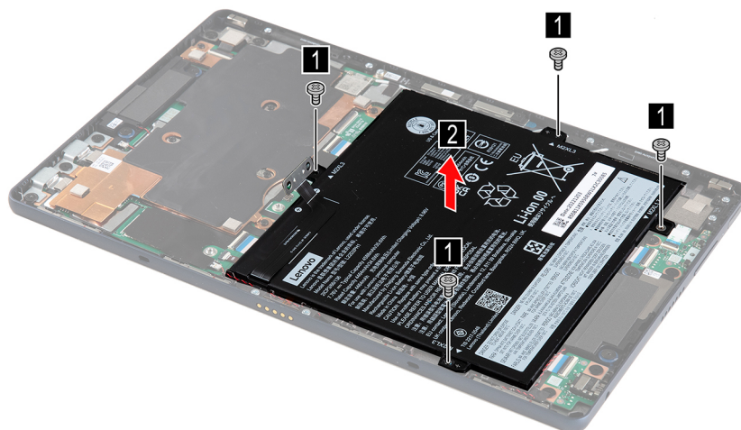
Figure 5. Remove the battery pack
