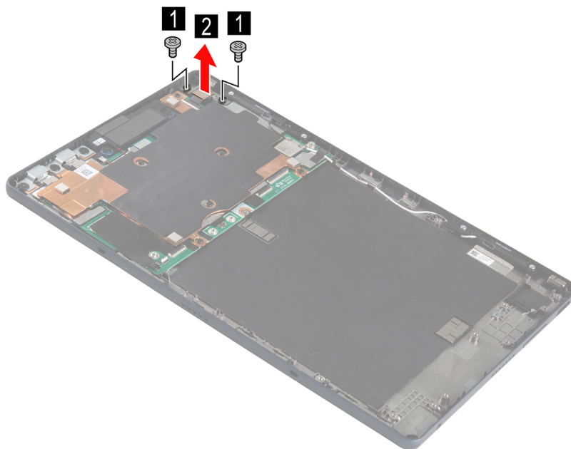
Figure 15. Remove the rear camera bracket
