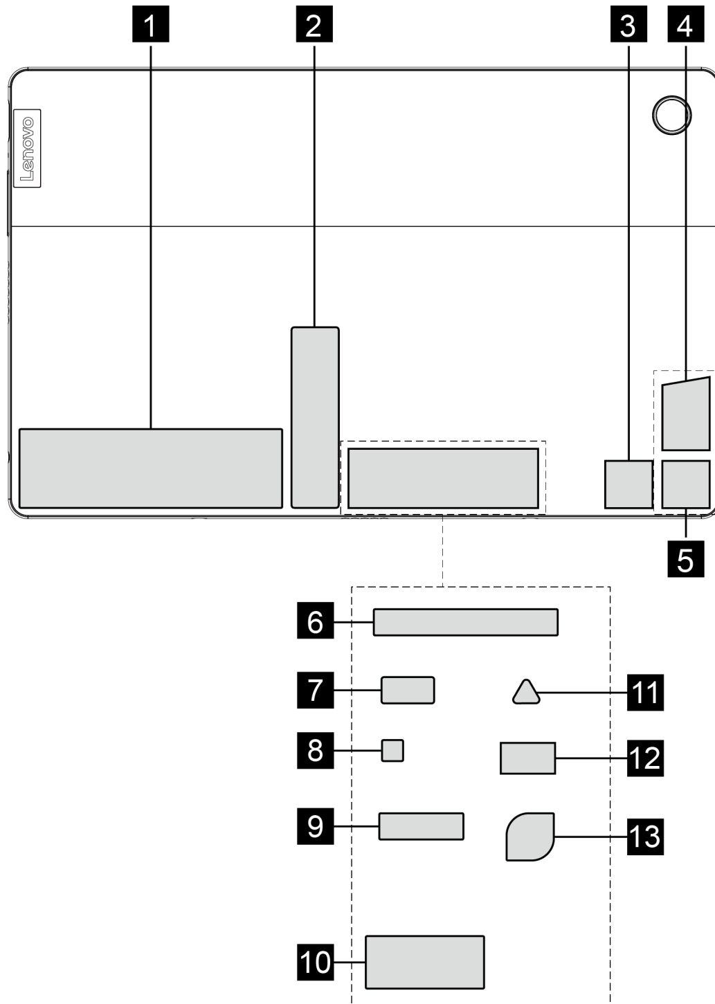
Figure 26. Label layout on the back side of the LCD cover
