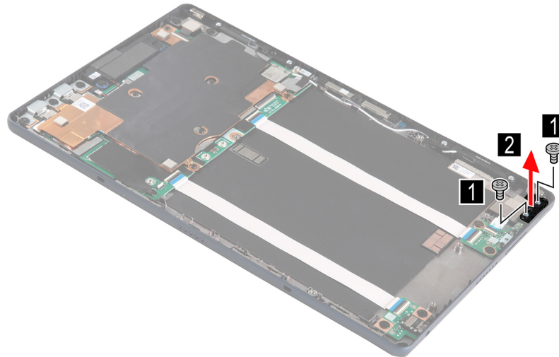
Figure 9. Remove two screws and the fingerprint board holder
