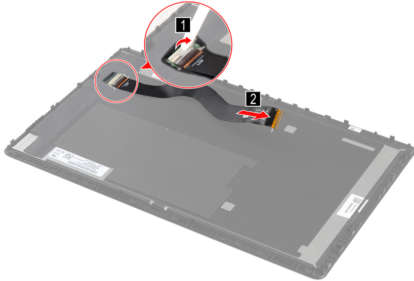
Figure 4. Remove the LCD cable
