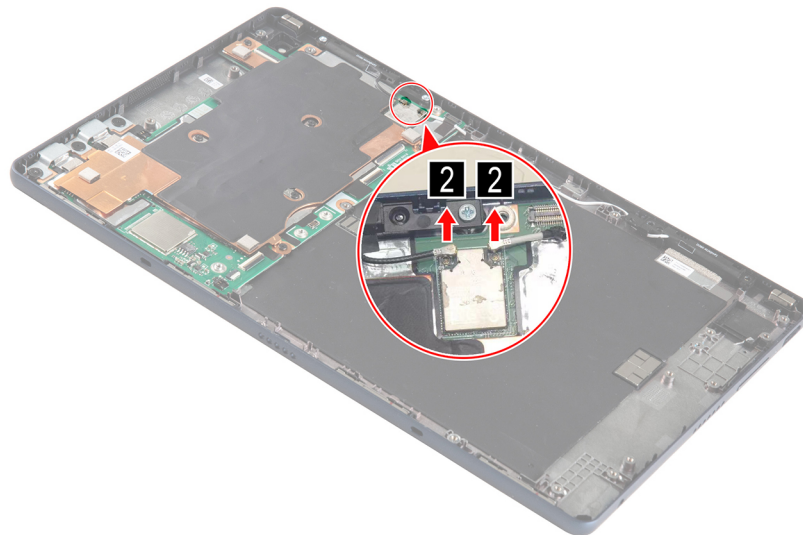
Figure 21. Disconnect the antenna cables from the system board
