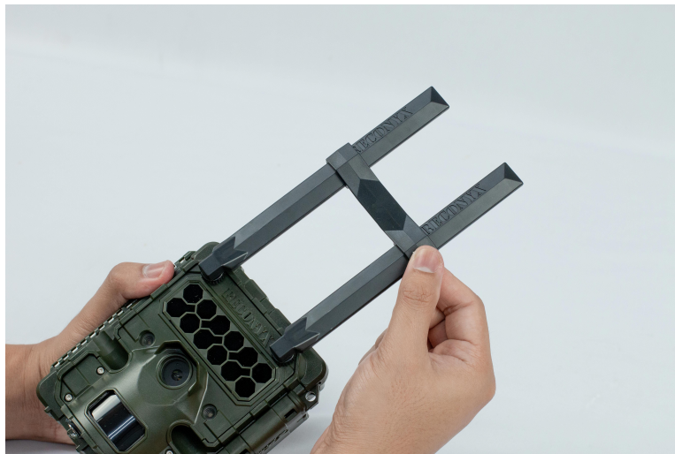
Figure 2: Slide in the Spreader Bar
