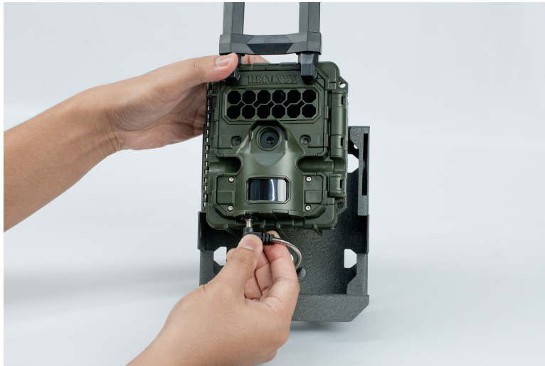
Figure 15: Plug in the Power Cable
