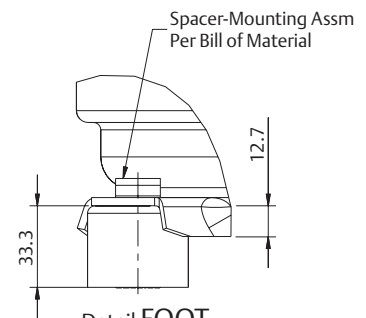
Detail FOOT Scale 1:1
