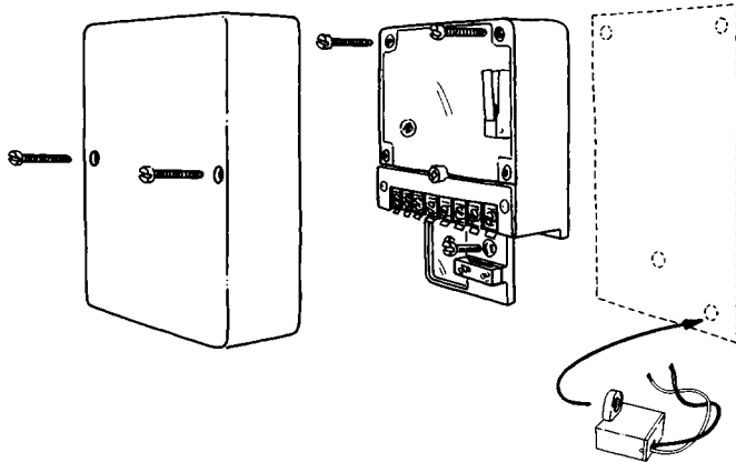
FIGURE 4 - MOUNTING DETECTOR ON A STEEL SURFACE
