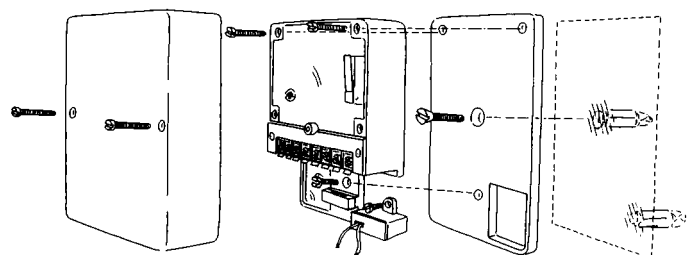
FIGURE 5 - MOUNTING THE DETECTOR ON CONCRETE
