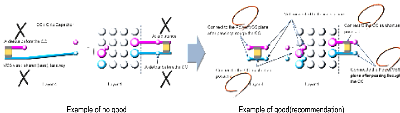
Figure 12, Image of recommended capacitor design for power supply and VCL (Layer 1 and 4, Top View)
