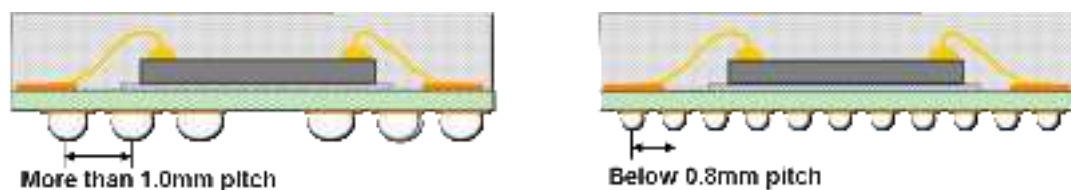
Figure 3, Definition of BGA and FBGA
