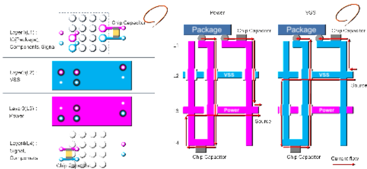
Example design of around the capacitor in each layer (Top View)
