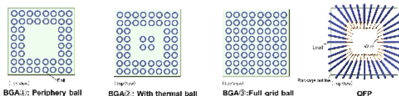
Figure 2, Example of BGA ball placement
