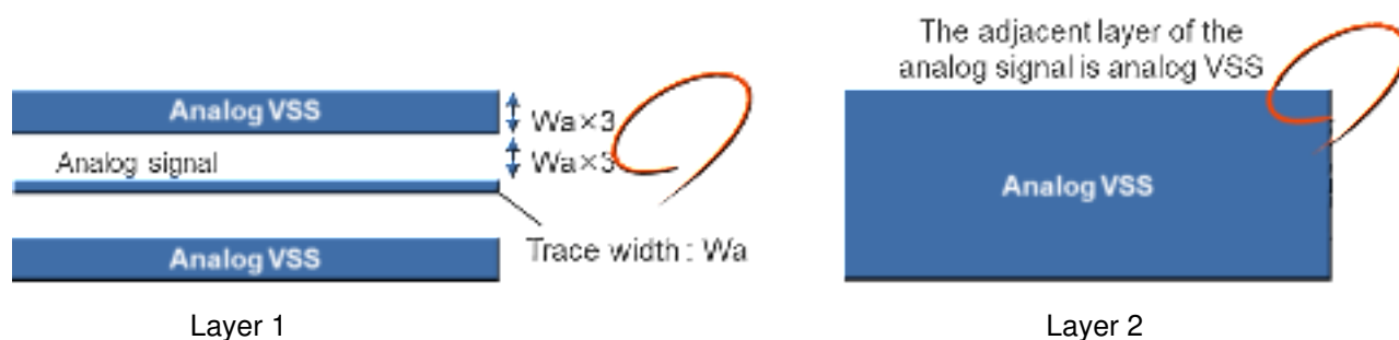
Figure 17, Recommended design image: Example of shielded trace (Top View)
