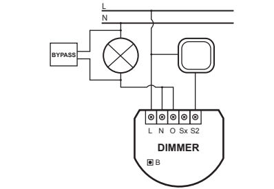
Fig.3 Wiring diagram for connecting the Bypass
