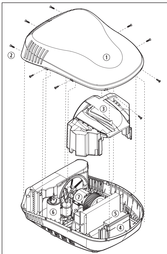
7 Blizzard NXT AC unit components and screw locations
