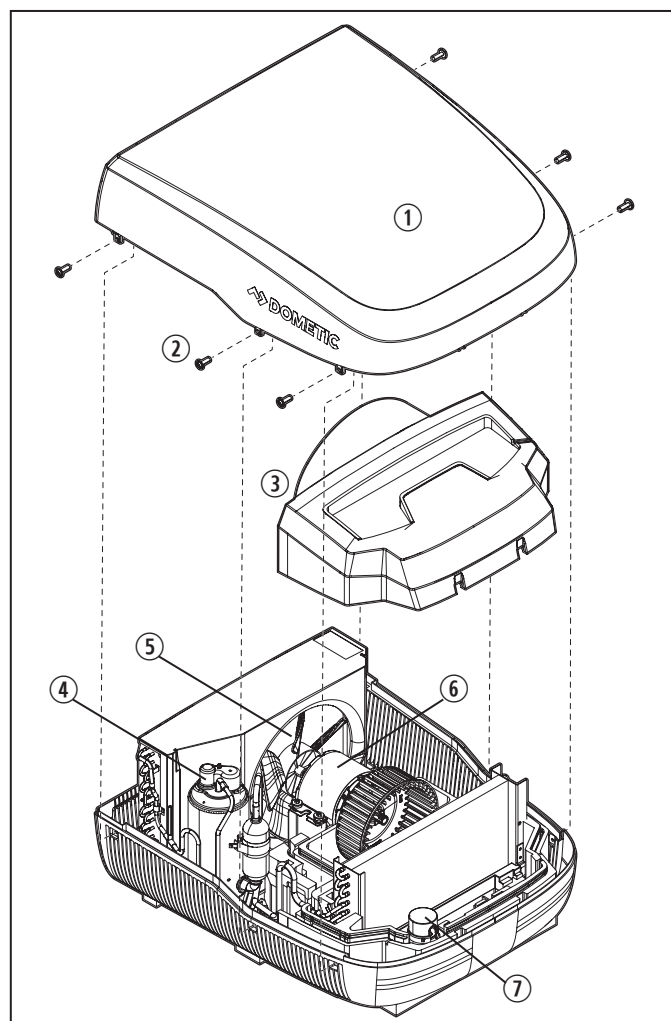
8 FreshJet AC unit components and screw locations
