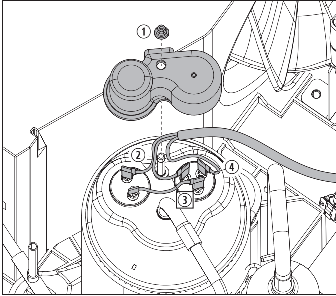
67 Compressor cap and factory wires
