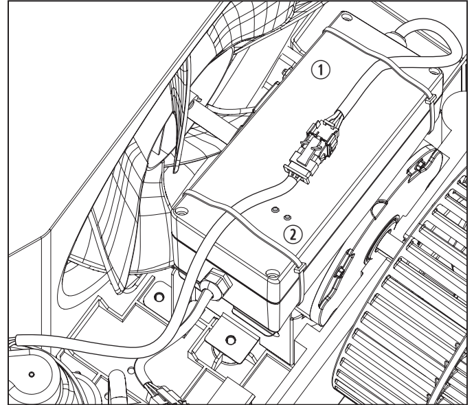
70 Compressor harness routed over the device
