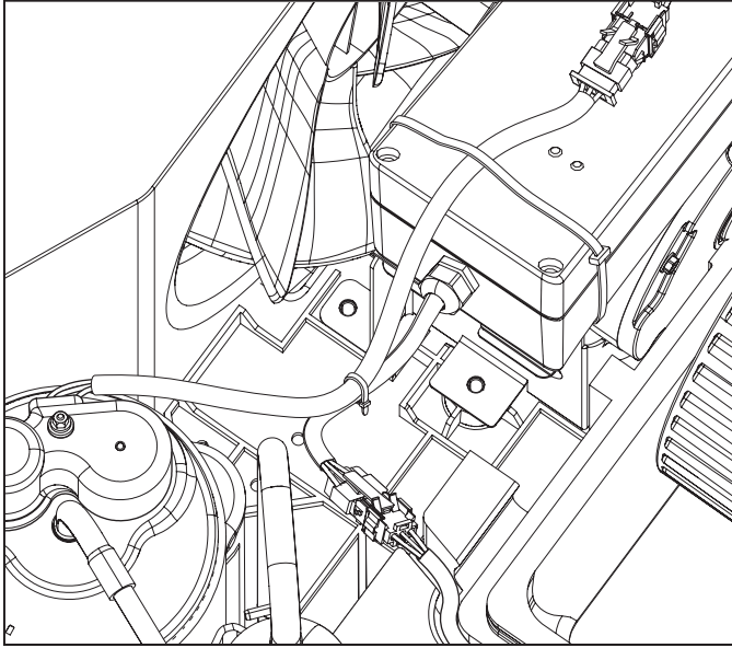
71 Compressor harness to supply harness
