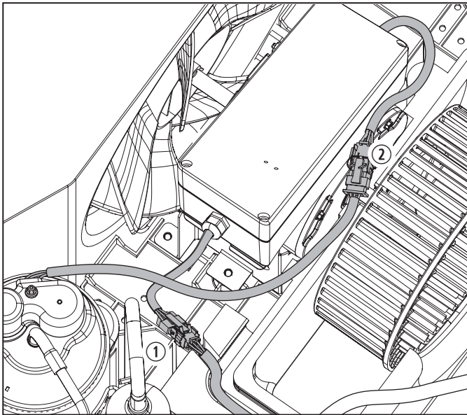
69 Supply and compressor harness connected to the device
