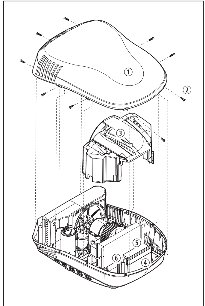
43 Removing the covers and foam
