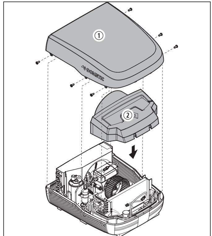
73 Replacement of foam and shroud
