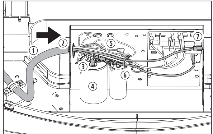
47 Connecting the wires
