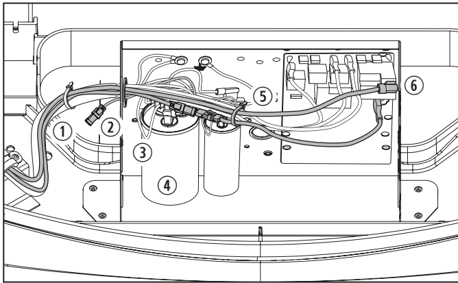
44 Disconnecting the compressor wires from the capacitor
