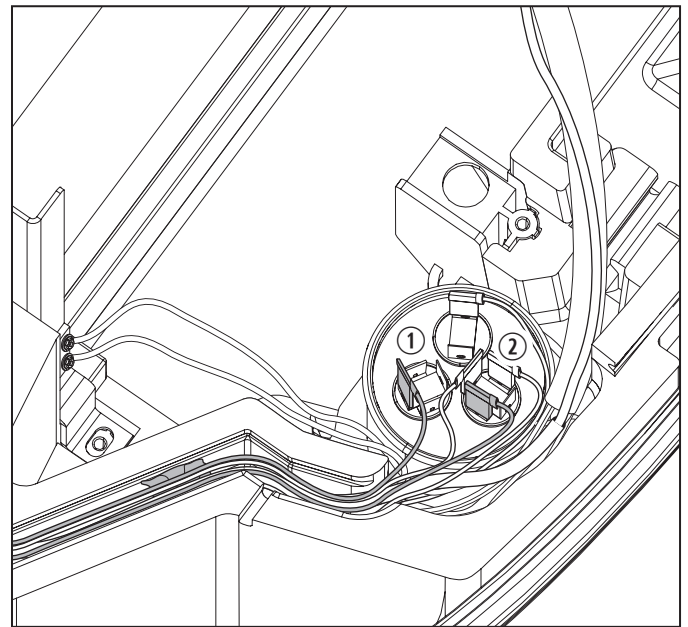
65 Attaching the device supply harness wires
