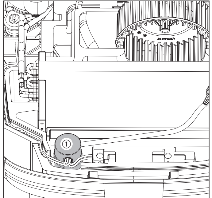
59 Capacitor location
