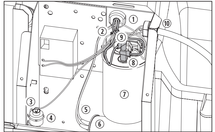
38 Disconnecting the compressor wires from the capacitor
