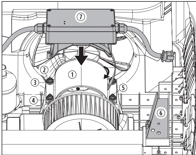
52 Placing the device on the fan motor
