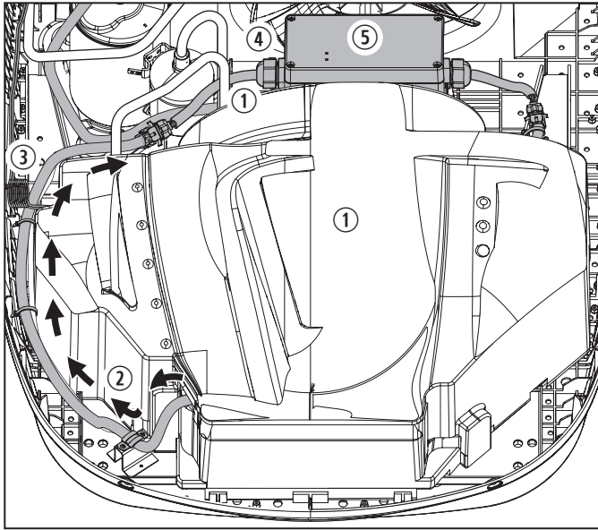
54 Connecting the harnesses to the device
