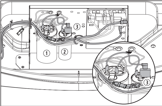
46 Disconnecting the motor starter
