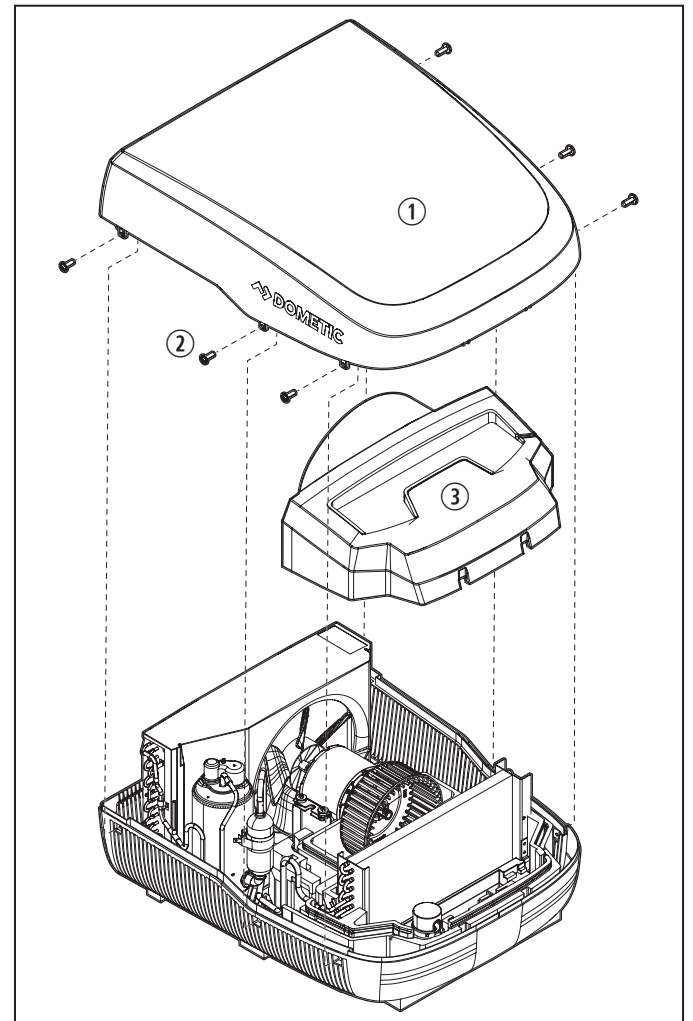
55 Removing the shroud
