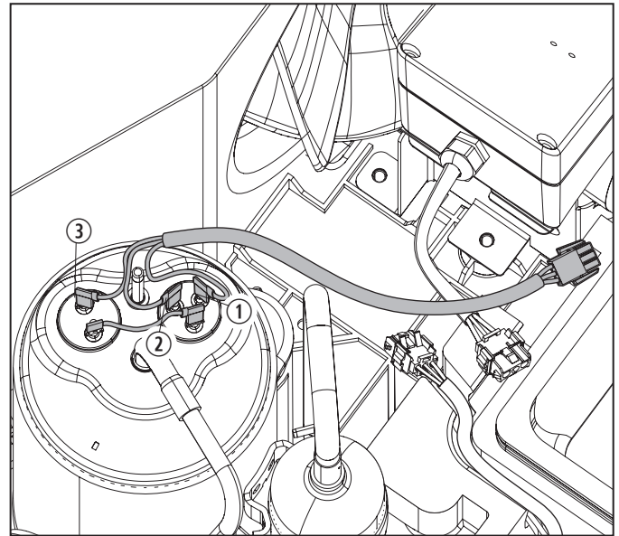
68 Compressor harness
