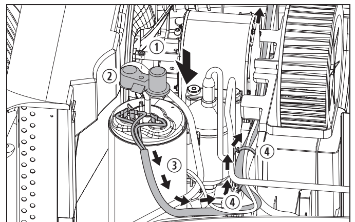
51 Routing the compressor wire harness
