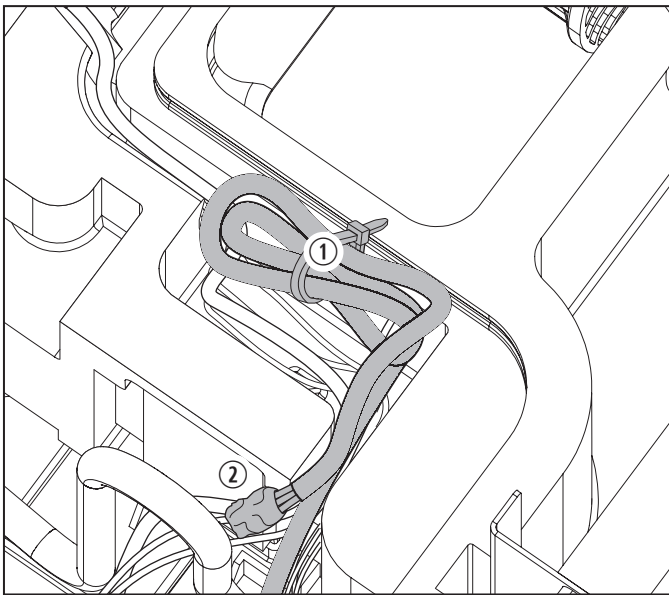
72 Factory Compressor Harness Wires Tapped and Bundled
