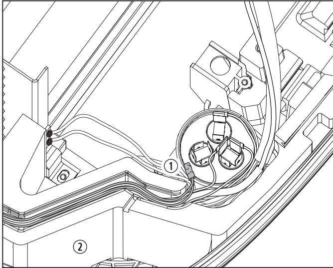
64 Removing the factory compressor wires
