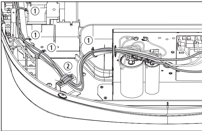
49 Securing the supply wire harness with new wire ties
