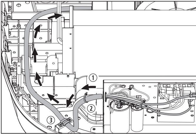
48 Routing the supply wire harness
