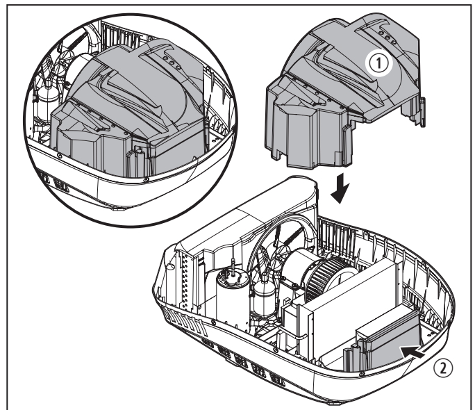
53 Replacing the foam shroud
