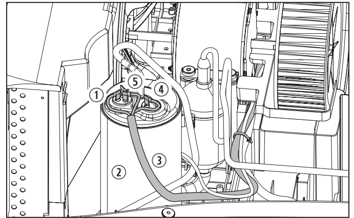
50 Connecting the compressor wire harness
