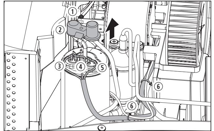
45 Disconnecting the compressor wires from the compressor
