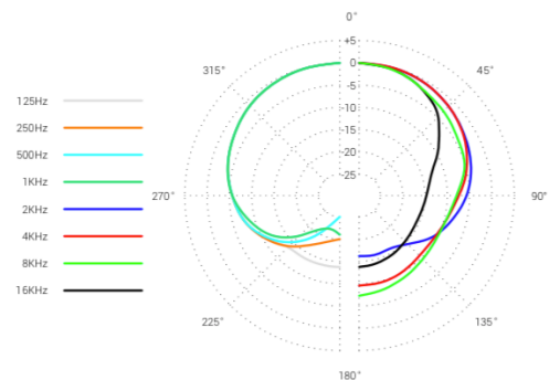
Polar Pattern
