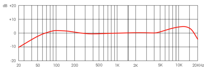
Frequency response
