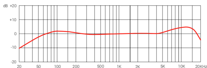
Frequenzgang
