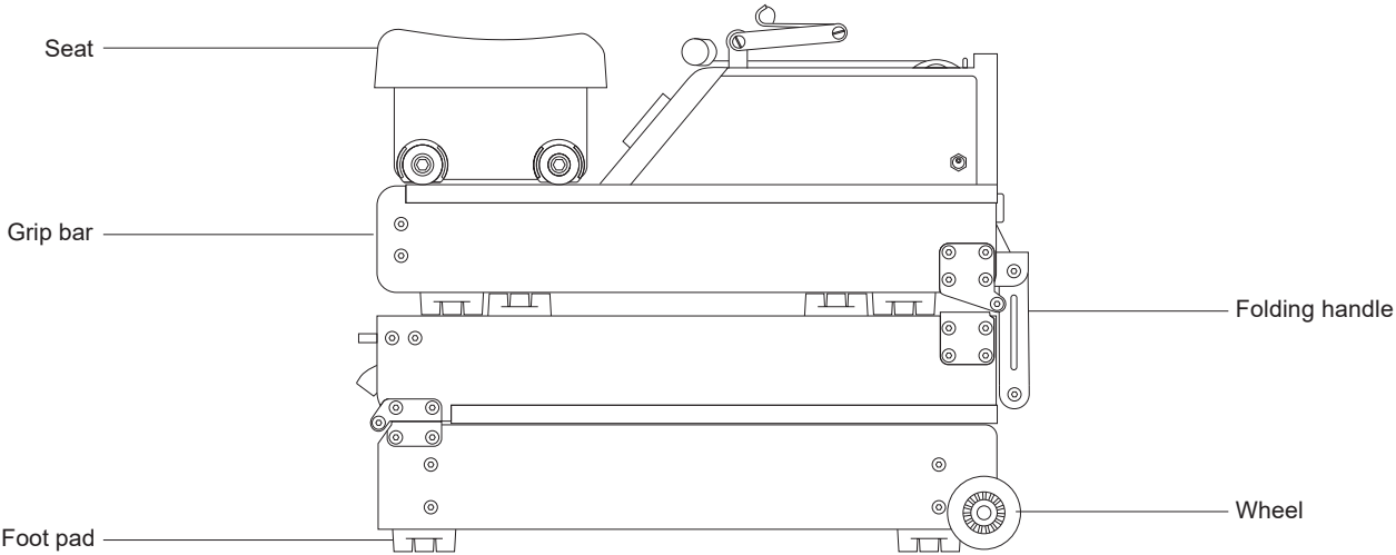
Folded state
