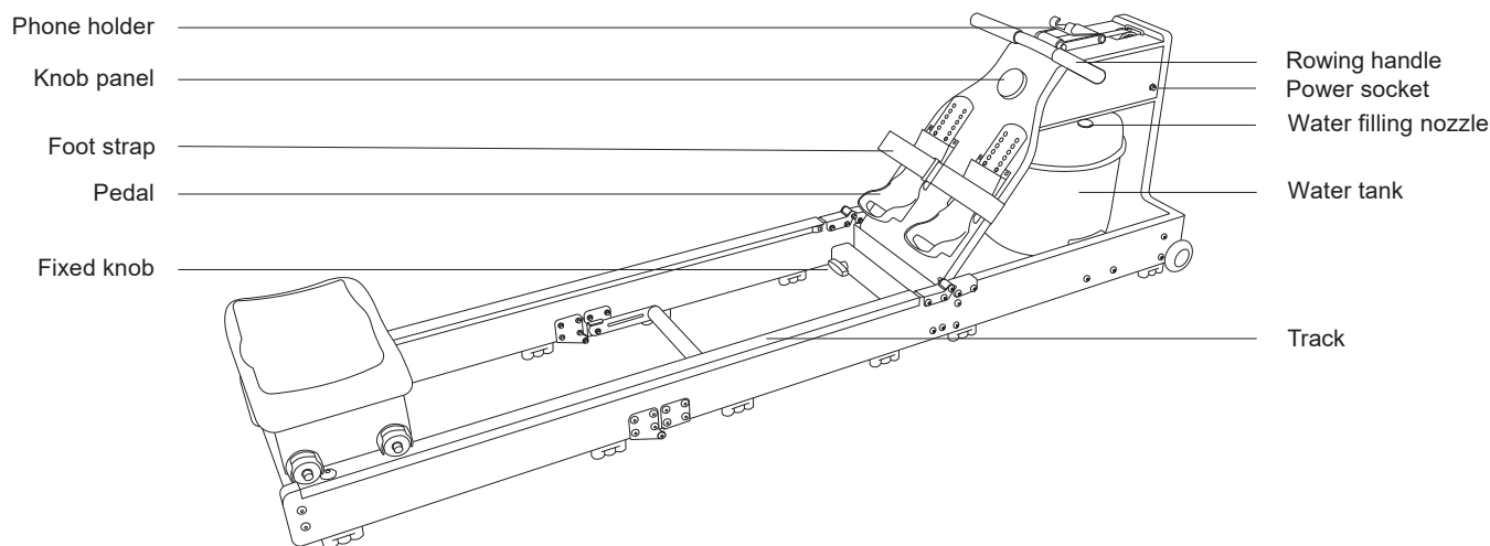
Unfolded state
