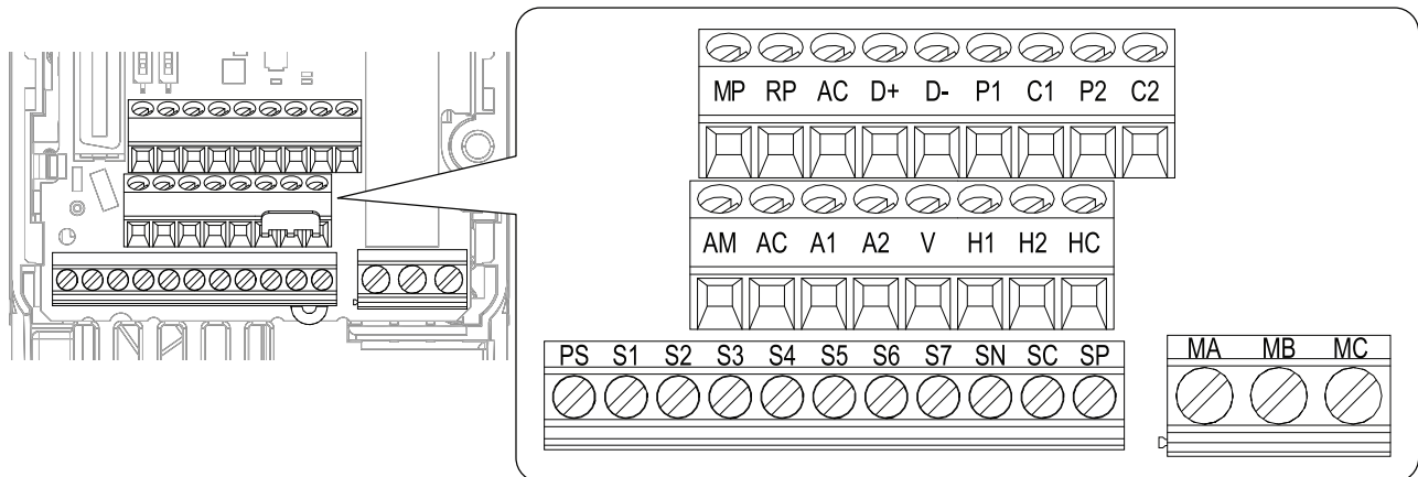
Figure 5 GA500 Control Circuit Terminals
