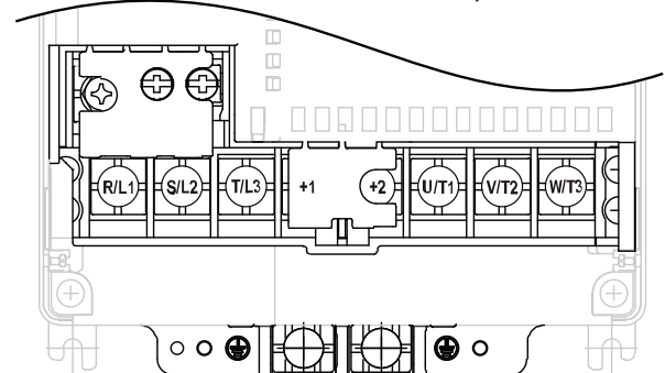
Figure 2 V1000 Main Circuit and Motor Circuit Terminal Layout by Model
